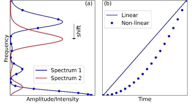
Fig. 2. (a) Reflection spectra (change of optical intensity as a function of optical frequency) at a given position before and after an environmental condition change. (b) Illustration of the laser frequency change over time, which is usually non-linear during the scanning.
