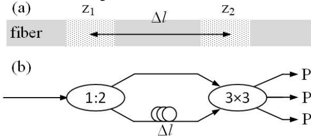
Fig. 1. (a) The phase difference between two positions determines the environmental condition, (b) schematic diagram of the imbalanced Mach-Zehnder interferometer used for phase retrieval.
