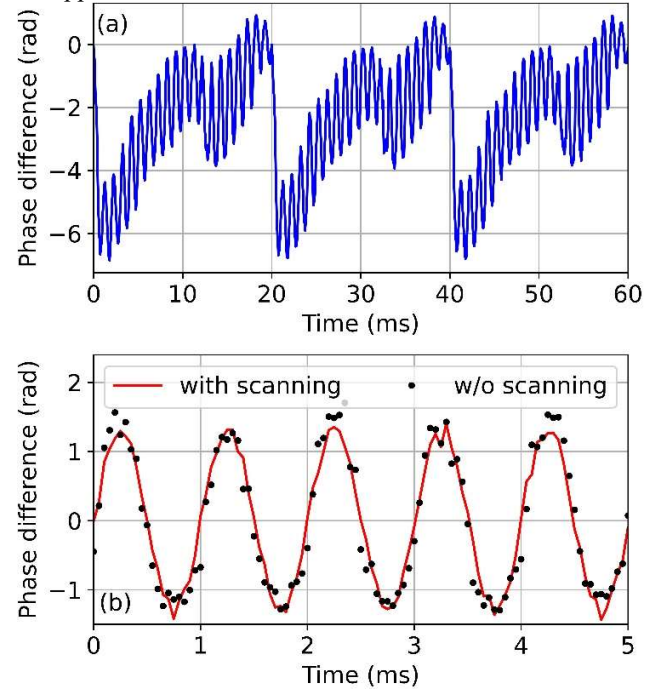
Fig. 5. (a) Optical phase demodulated at the perturbed fiber section. (b) comparison of the filtered phase and the modified phase obtained by the \phi OTDR system based on the IMZI scheme with and without frequency scanning, respectively. [13]
