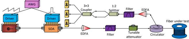
Fig. 4. Proposed \phi OTDR system that employs an optical frequency scanning laser and an imbalanced Mach-Zehnder interferometer.
