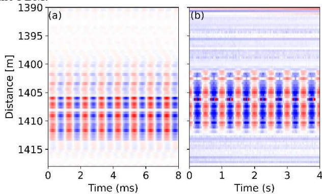
Fig. 8. Waterfall diagrams of the vibration measured by (a) phase-based method and (b) amplitude-based method.
