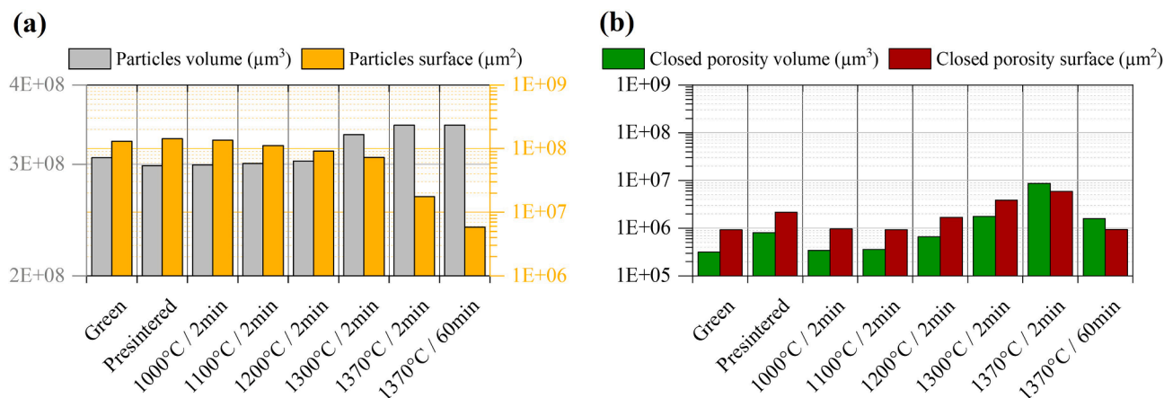
Fig. 4. (a) Measured particles (material skeleton) and (b) closed porosity volume and surface area for each sample dataset analyzed. Note that open porosity was excluded by eliminating the largest pore on each dataset.
