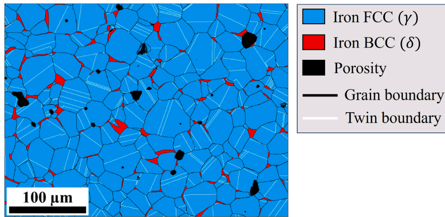
Fig. 16. EBSD phase map from the cubical sample sintered up to 1370 °C for 1 h, where FCC austenite (blue), BCC \delta -ferrite (red) and porosity (black) phases are shown. The grain boundaries and twin boundaries are shown as black and white lines, respectively.
