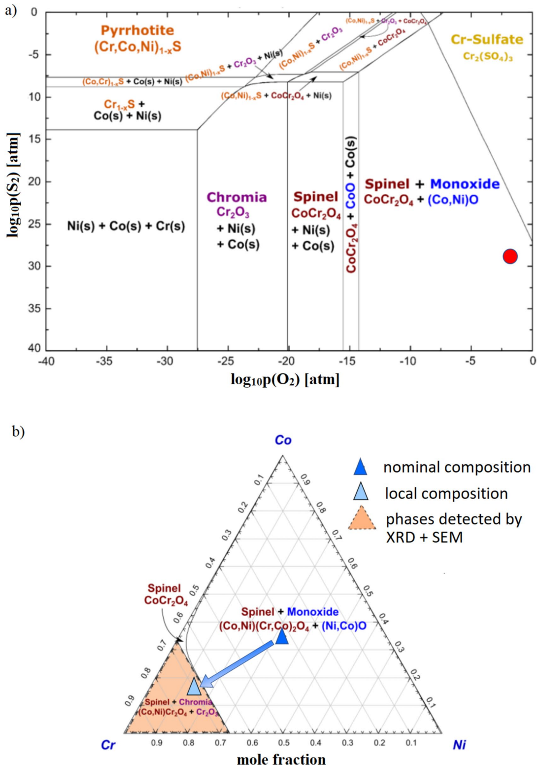
Fig. 9 a \log(p_{\text{O}_2}) vs. \log(p_{\text{S}_2}) plot for the equimolar CrCoNi MEA at p_{\text{H}_2}=10^{-9} atm and 800 °C. The filled red circle represents the p_{\text{O}_2} and p_{\text{S}_2} at the gas/oxide interface. b Stability diagram for the formation of oxides in the Cr–Co–Ni system with a constant partial pressure of \text{O}_2 , \text{S}_2 (directly linked to \text{SO}_2 ) and \text{H}_2 (directly related to
