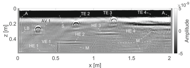
Fig. 8 Elastic SH RTM result obtained using the migration model presented in Fig. 7 (AV 1: first cavity, TE 2, TE 3 and TE 4: top edges of the second, third and fourth cavity, VE 1: vertical edge of the first step, HE 1, HE 2, HE 3 and HE 4: lower boundary of the concrete layer at different depths, LB: left lateral boundary of the concrete layer, A and M: migration artefacts)
