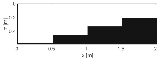
Fig. 13 Structure of the velocity and density model used for the fourth elastic SH RTM (taken from [51])
