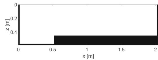
Fig. 9 Structure of the velocity and density model used for the second elastic SH RTM (taken from [51])
