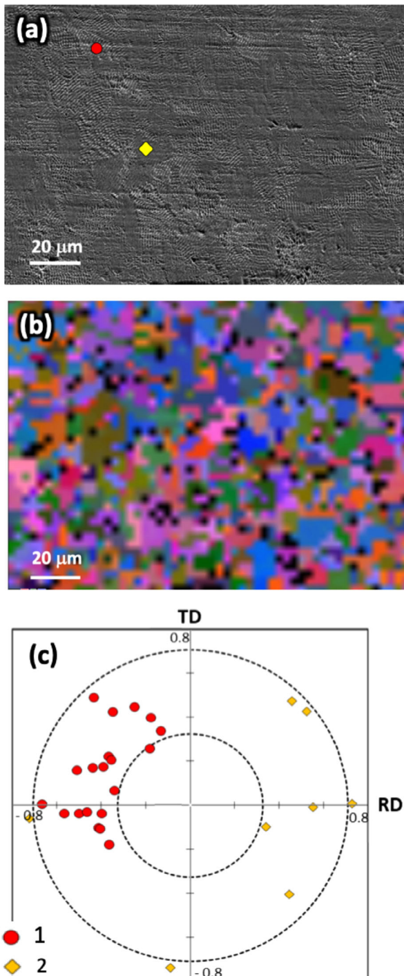
Figure C1. a) SEM micrograph (SE) of a SS316L surface treated with an 800 ps IR ( \lambda = 1064 nm) laser (sample was tilted at \alpha = 70^\circ for EBSD analysis). The laser processing parameters are: f_{rep} = 300 kHz, E_{pulse} = 14.7 \mu J, v_{laser} = 1500 mm s^{-1} and \delta_{lines} = 3 \mu m. b) EBSD Euler map of the same area. c) RD-TD grain orientation map. Each symbol corresponds to an analyzed grain showing well-defined ripples ( \Lambda \approx 1 \mu m) (Nanostructure type 1) or a nanostructure with emerging ripples (Nanostructure type 2). The axes values are given in units of e .
