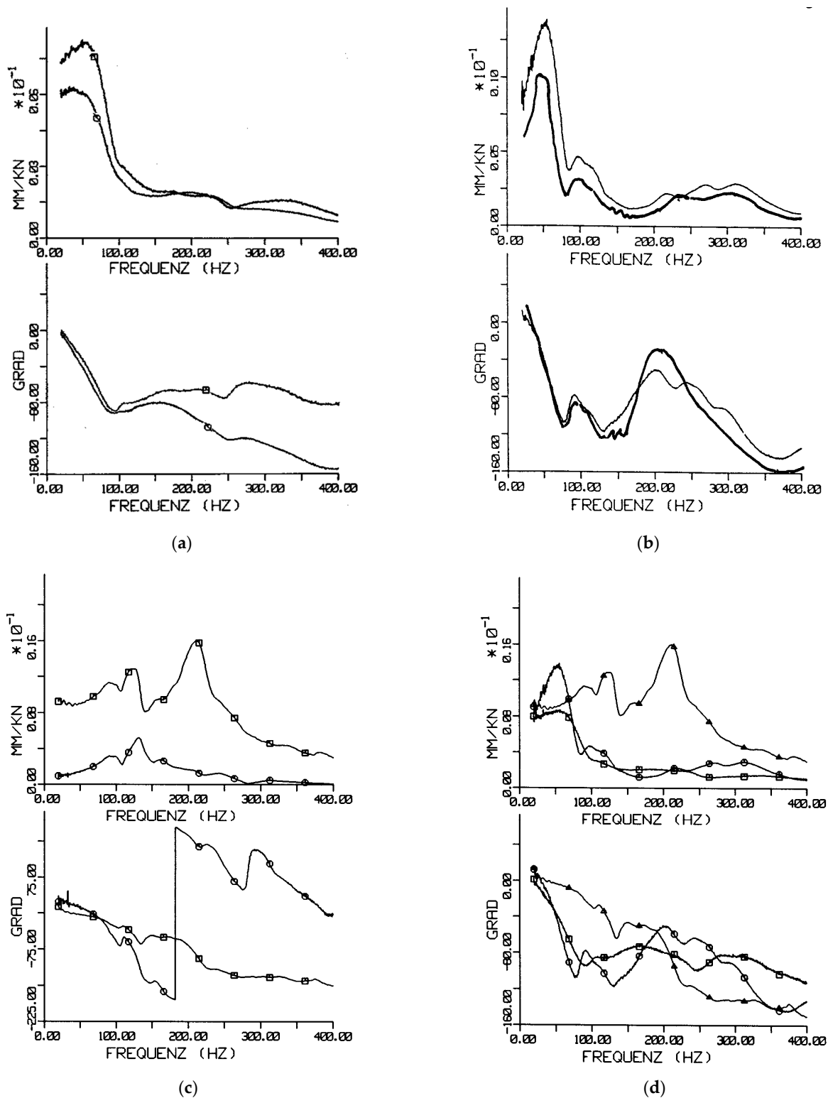
Figure 15. Compliances of the rail (□) and sleeper (○) of the different tracks, (a) on the soil, (b) on the bridge, (c) in the tunnel, and (d) comparison of the rail compliance for the ballasted track □ on the soil, ○ on the bridge and △ the slab track in the tunnel.
