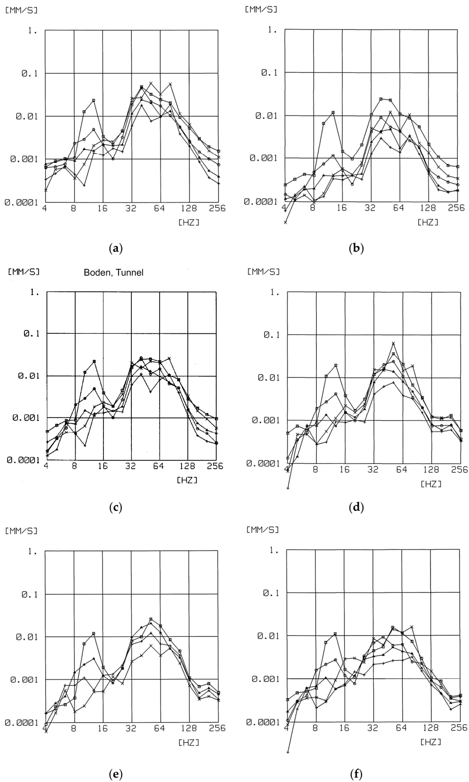
Figure 8. Vibrations of the soil above the tunnel at horizontal distances of (a) 3 m, (b) 5 m, (c) 10 m, (d) 20 m, (e) 30 m and (f) 50 m, one-third octave band spectra for different train speeds: □ 160, ○ 125, △ 100, + 80, × 63 km/h.
