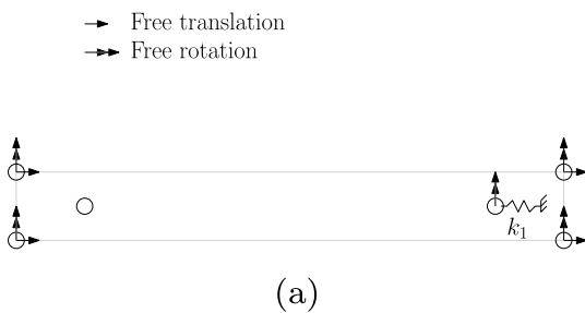
Fig. 12. Third boundary condition configuration, which considers a linear spring k_1 in the longitudinal direction of the FEM of the Folke Bernadotte Bridge.
