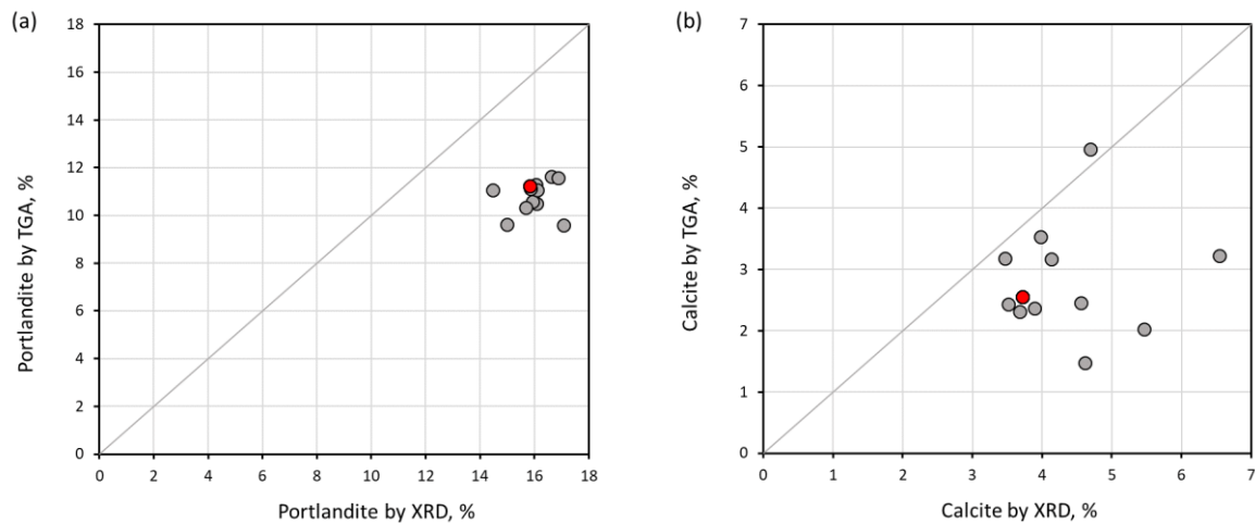
Figure 11. Comparison of the results obtained by XRD and TGA: (a) portlandite content; (b) calcite content.
