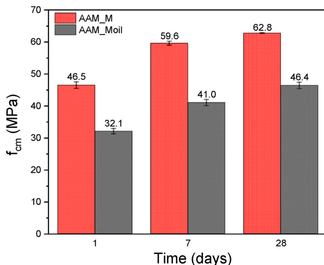
Fig. 2. Compressive strength ( f_{cm} ) development of AAM_M and AAM_Moil with time.
