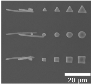
Figure 7. SEM image of rod feature (#4) directly on the substrate, partially collapsed are the smallest three rods of each geometry, SZ2080, 6 mW, d_h 0.2 \mu\text{m} , d_z 0.4 \mu\text{m} , 3DPoli sliced.
