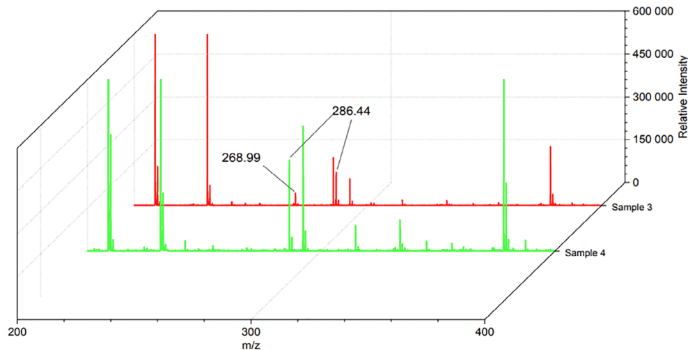
Figure 2 Positive ion MALDI-TOF mass spectra of flavonoid sum from L. pratensis L. Representation of m/z value of spot zones (sample 3 with R_f = 0.2 , sample 4 with R_f = 0.59 ).
