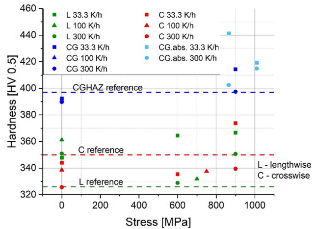
Fig. 7 HV0.5 hardness dependent on microstructure, heating rate, and applied stress
