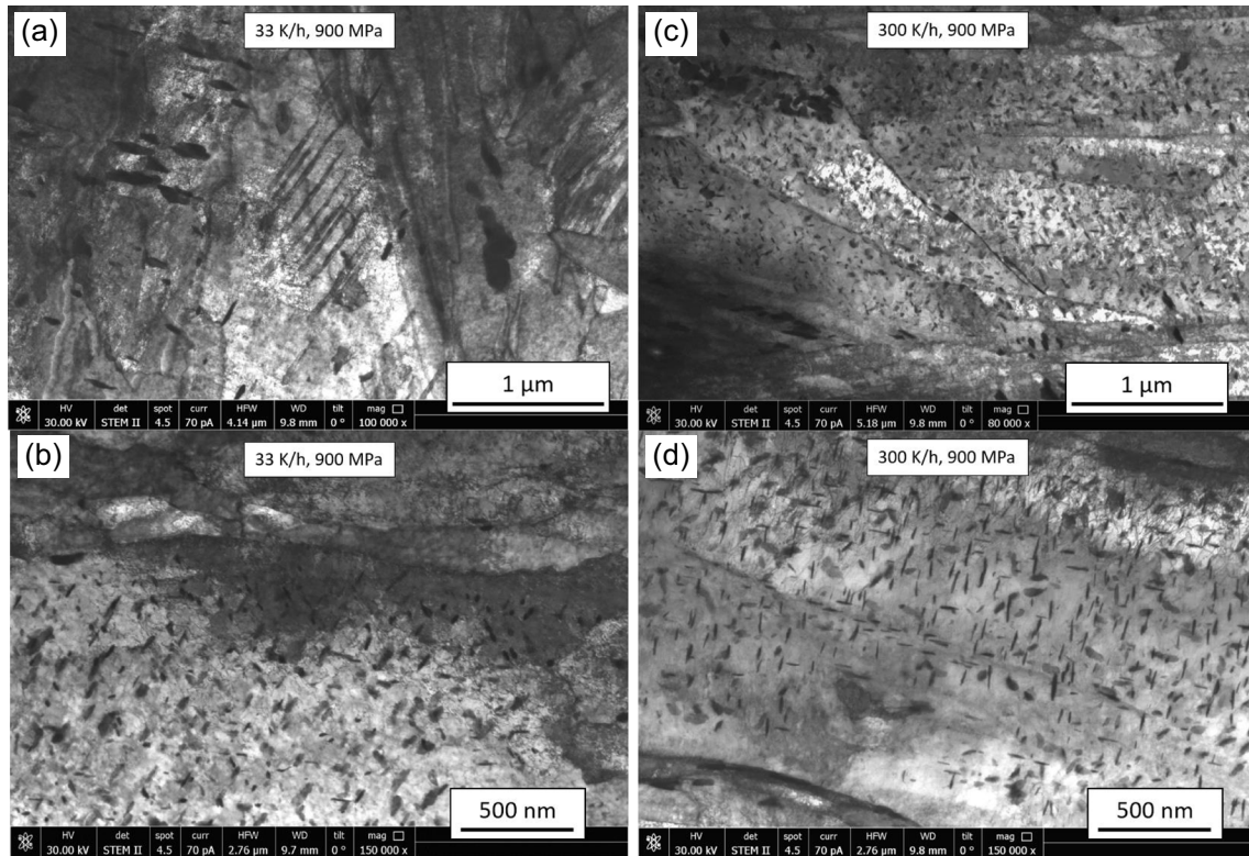
Fig. 6 Scanning transmission electron microscopy (STEM) comparison of simulated CGHAZ microstructures after different PWHT treatments: a, b \phi = 33 K/h, T_{end} = 500 °C and 900 MPa, c, d \phi = 300 K/h, T_{end} = 500 °C and 900 MPa
