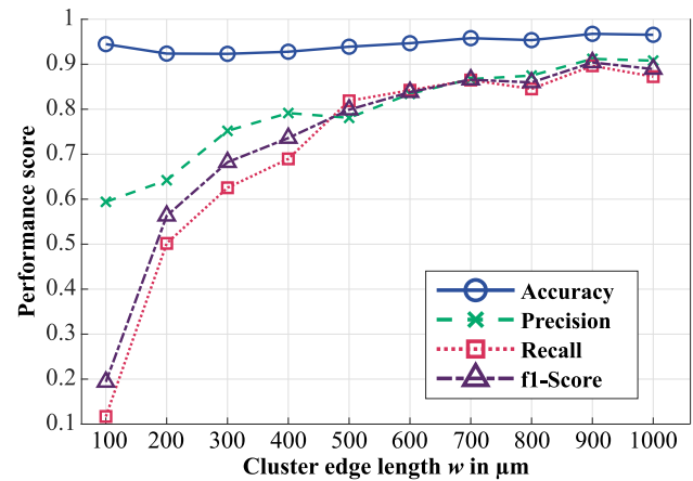
Fig. 10 Influence of cluster dimension on model performance for a porosity threshold of 0.1\% and considered voxels from N = 9 subsequent layers
