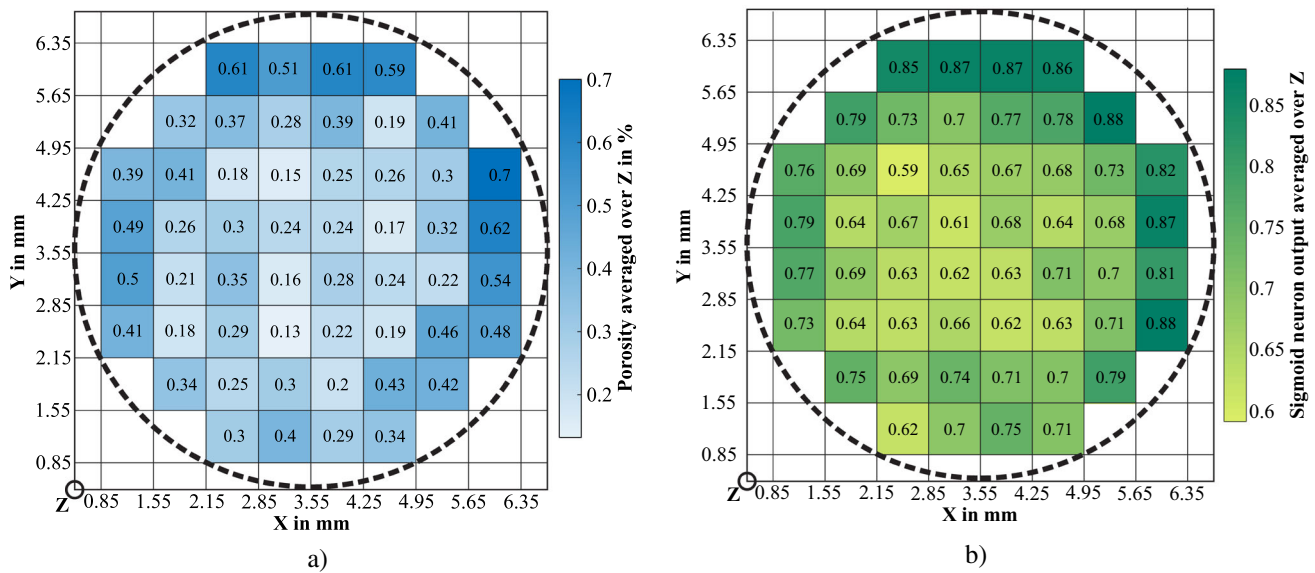
Fig. 13 Porosity vs. raw model prediction averaged along the Z axis from 6.5 to 7.5 mm. In this area, a major part of “porous” clusters was located resulting from the VED increase in component sections 3, 4 and 6. The dashed line indicates the outer rim of the cylindrical specimen. a Average porosity per target voxel. b Average output of sigmoid
