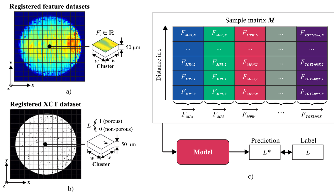
Fig. 4 Data pre-processing for the generation of samples. a Resampling of thermogram feature data to larger clusters with an edge length w and a height of 50 \mu\text{m} . Shown here is a 2D feature slice extracted from the MPA dataset. b Resampling of XCT dataset to larger clusters. The label L is calculated based on the porosity threshold P_{thresh} (see “Sample
