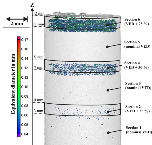
Fig. 12 Visualization of the void distribution of the XCT data. Component sections of applied increased VED are highlighted. The equivalent void diameter is indicated by the color and corresponds to the diameter of a sphere with similar volume. The component sections are indicated by the dashed lines. Pores belonging to the contour scan are blanked out for increased visibility
