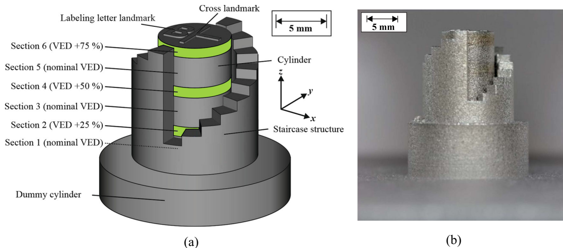
Fig. 2 Component design inspired by a study by Gobert et al. (2018) as computer-aided design (a) and after manufacturing (b). The specimen was manufactured from AISI 316L stainless steel. The outer staircase and the landmarks positioned on the specimen top were utilized for registration purposes (Oster et al., 2022). In the green component section
