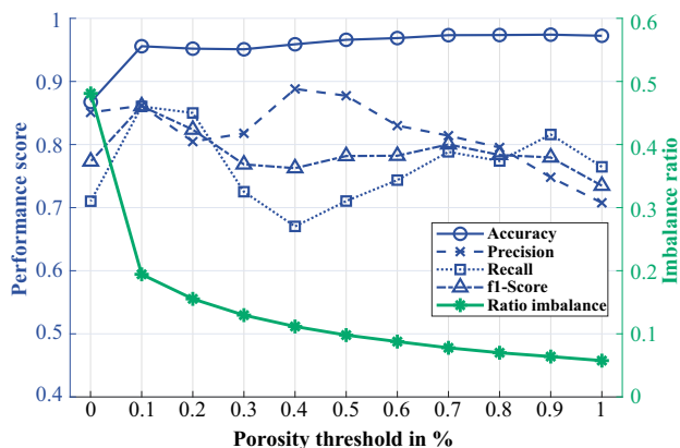
Fig. 9 Model performance depending on the set porosity threshold and imbalance ratio between both classes for a cluster dimension of (700 \times 700 \times 50) \mu\text{m}^3 and nine included subsequent layers
