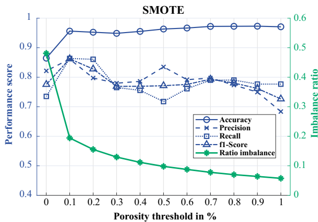
Fig. 15 Model performance in dependency on the chosen porosity threshold with application of SMOTE sampling method. The performance scores remain comparably similar for the usage of SMOTE in comparison to the original dataset
