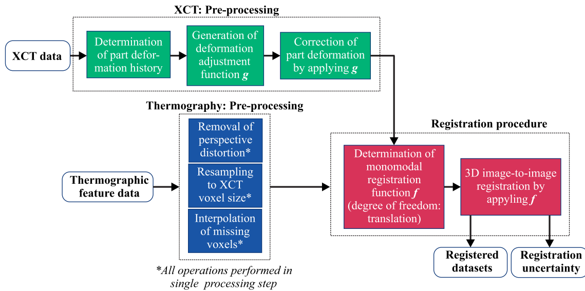
Fig. 3 Flow chart of the registration process of XCT data and thermographic feature data
