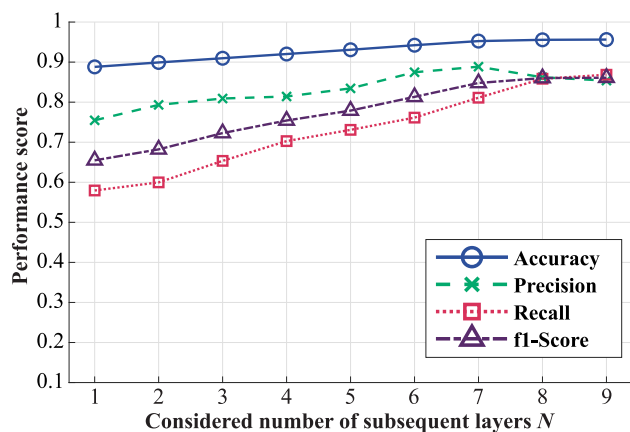
Fig. 11 Influence of considered number of subsequent layers on model performance for a porosity threshold of 0.1% and a target voxel size of (700 \times 700 \times 50) \mu\text{m}^3
