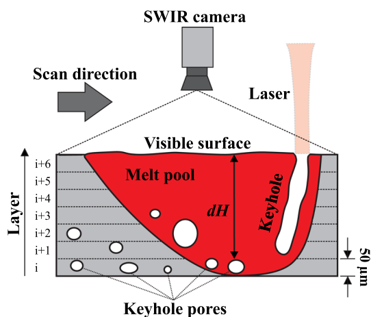
Fig. 5 Schematic keyhole pore formation with height difference dH between the part surface and forming keyhole pores at the bottom of the melt pool
