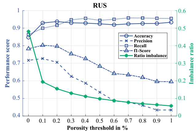
Fig. 16 Model performance in dependency on the chosen porosity threshold with application of RUS sampling method. In comparison to SMOTE and the original dataset the application of RUS result in very high recall scores, while f1-Score and precision are significantly lower
