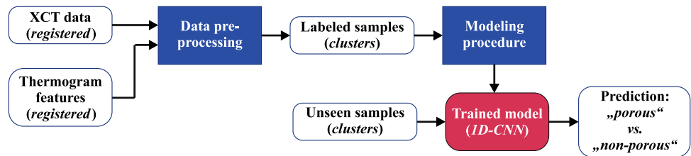
Fig. 1 Illustration of framework for the cluster-wise prediction of local porosity
