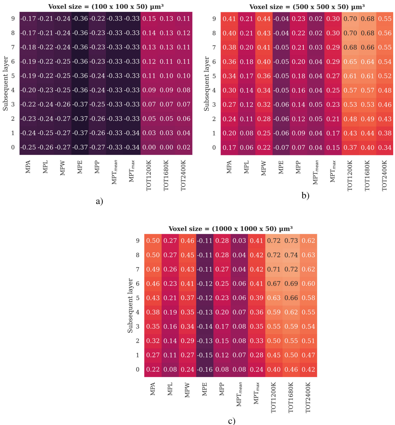
Fig. 8 Correlation coefficients between labels and features determined for three different sets of cluster dimensions. The extracted thermographic features are given on the abscissa and the voxel position above the label is shown on the ordinate
