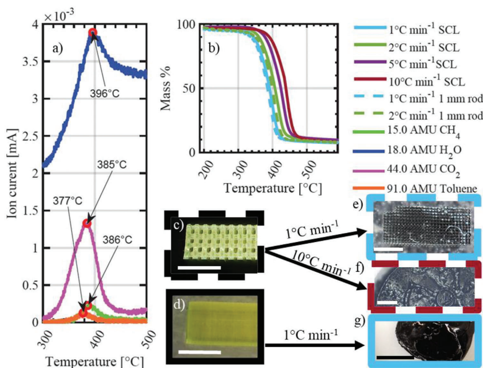
Figure 2. a) Mass spectrum of the gas fraction of an SCL fragment heated at 5\text{ °C min}^{-1} . The temperatures at which the maximum abundance of the detected volatiles occur are denoted with red circles. b) Thermogravimetric analysis (TGA) of four simple cubic lattices (SCL) and two rods. The mass percentage versus temperature at four different heating rates from 25 to 600\text{ °C} and two sample geometries of 2PP printed UpCarbon are displayed. c) SCL prior to carbonization. d) 1 mm rod prior to carbonization. e) SCL after a 1\text{ °C min}^{-1} heating rate. f) pitch like residue resulting from a 10\text{ °C min}^{-1} heating rate of a SCL. g) Pitch like residue of a 1 mm rod heated at 1\text{ °C min}^{-1} . Subfigure (c–f) illustrates how the process is sensitive to heating rate and scale. All scale bars are 1 mm.
