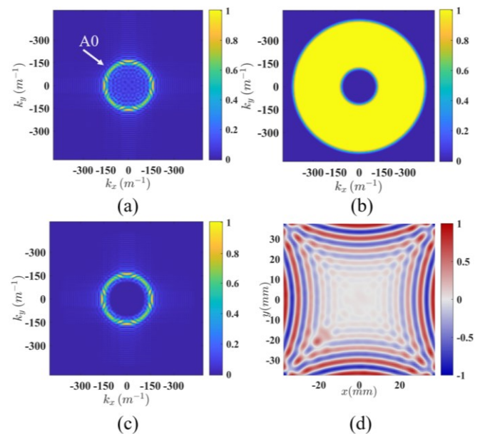
Fig. 6. Frequency-wavenumber filtering process in the cartesian coordinate: (a) amplitudes in wavenumber domain, (b) filter mask, (c) filtered amplitudes in wavenumber domain and (d) corresponding filtered wavefield.
