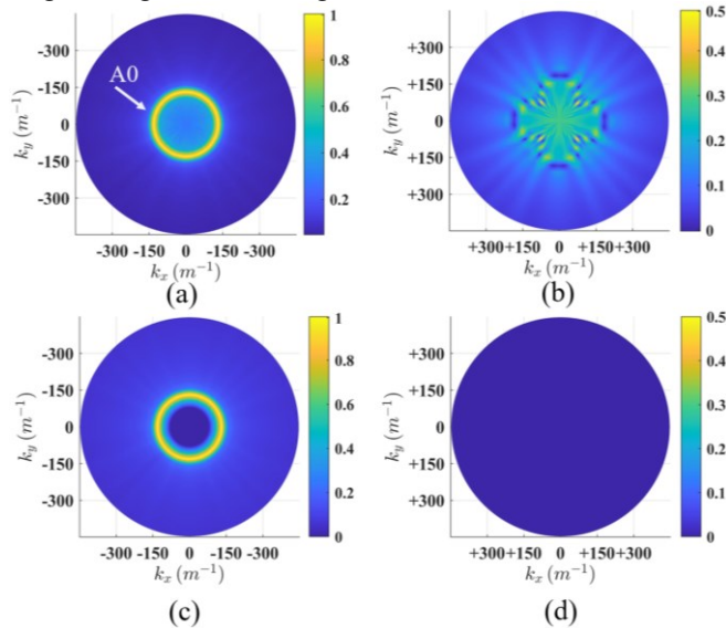
Fig. 4. Frequency-wavenumber filtering process in the polar coordinate: (a) negative wavenumber of the incident wave, (b) positive wavenumber of the reflected wave, (c) filtered wavenumber of the incident wave and (d) filtered wavenumber of the reflected wave.
