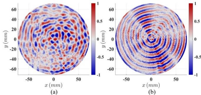
Fig. 12. Normalized wavefields measured by 3D LDV at time t = 113.92 \mu s on the adhesively bonded aluminum specimen: (a) unfiltered wavefield and (b) filtered wavefield.
