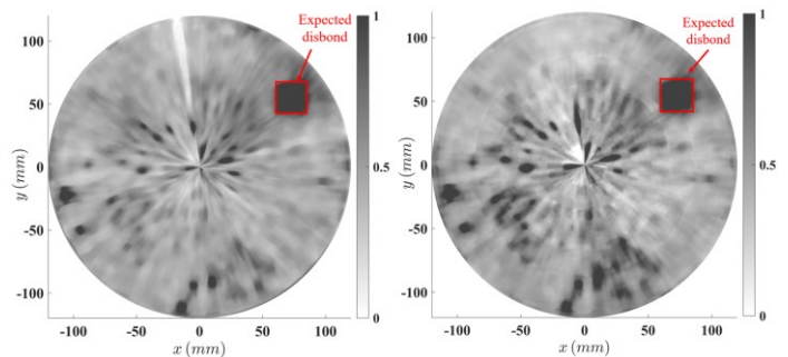
Fig. 16. Damage imaging results of the 3D LDV measurement on the bonded CFRP plate using (a) RMS* and (b) ED*.
