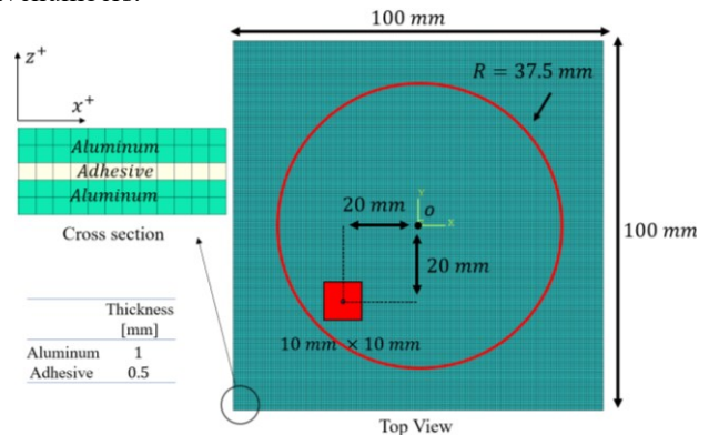
Fig. 2. Schematic of the meshed adhesively bonded aluminum plate model, disbond location, and scan area.
