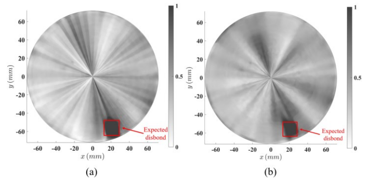
Fig. 13. Damage imaging results of the 3D LDV measurement on the bonded aluminum plate using (a) RMS* and (b) ED*.
