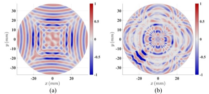
Fig. 5. Normalized wavefields at a time instant t = 44.75 \mu s of the numerical simulation: (a) unfiltered data and (b) frequency-wavenumber filtered data.
