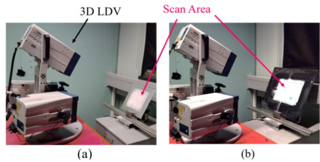
Fig. 10. 3D LDV measurement set-up of the bonded specimens: (a) adhesively bonded aluminum specimen and (b) adhesively bonded CFRP plate.
