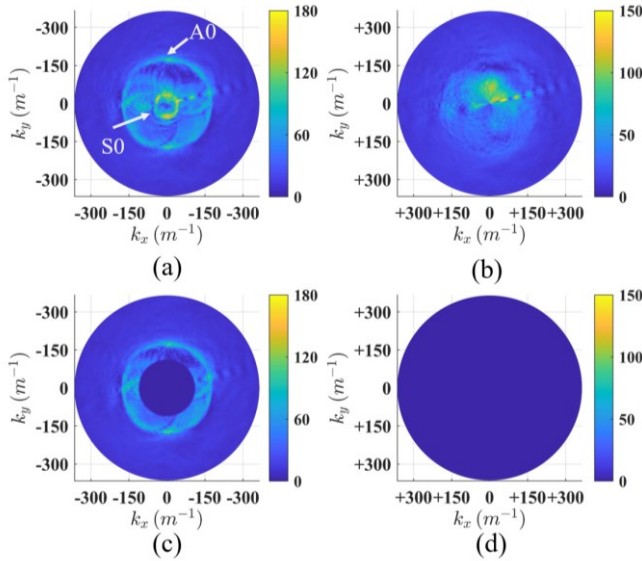
Fig. 14. Frequency-wavenumber filtering process on the 3D LDV measurements for the bonded CFRP plate: (a) negative wavenumber of the incident wave, (b) positive wavenumber of the reflected wave, (c) filtered wavenumber of the incident wave and (d) filtered wavenumber of the reflected wave.
