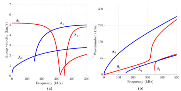
Fig. 1. Dispersion curves for the adhesively bonded sample used in the numerical model: (a) group velocities and (b) wavenumbers.
