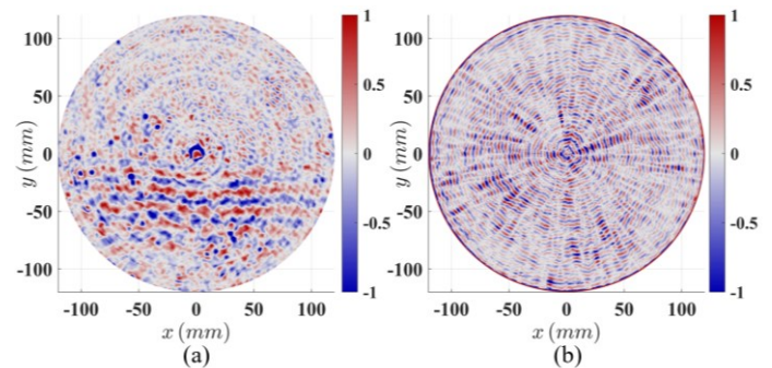
Fig. 15. Normalized wavefields measured by 3D LDV at a time instant t = 176.32 \mu\text{s} on the adhesively bonded CFRP specimen: (a) unfiltered wavefield and (b) frequency-wavenumber filtered wavefield.
