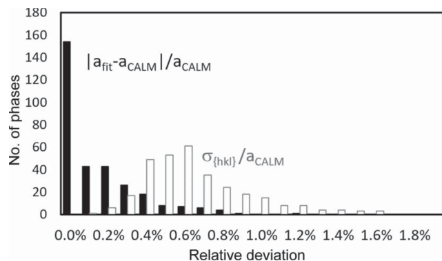
Figure 4 A comparison between the deviation of the relative lattice parameters derived using CALM and corrected with equation (3), and the band width-related standard deviation \sigma_{hkl} .
