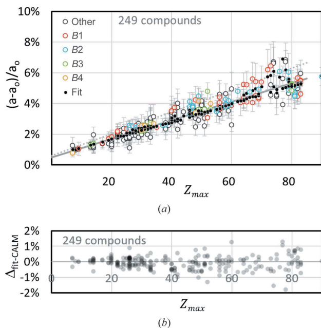
Figure 8 (a) The offset distribution as a function of Z_{\max} for 249 compounds, displayed as hollow circles. For comparison, the light-grey dotted line indicates the offset level displayed in Fig. 2. The black dots represent the offset according to equation (3) with Z = Z_{\max} . (b) A plot highlighting the differences between the hollow circles and the respective black dots.
