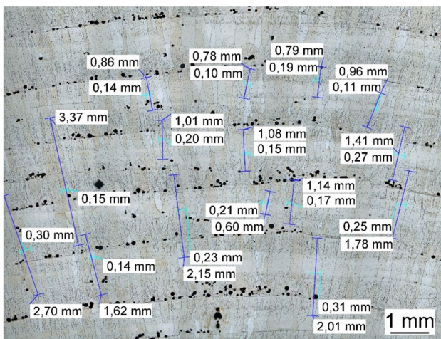
Fig. 6 Exemplary grain measurement of Alloy 36+0.33 wt.-% Ti
