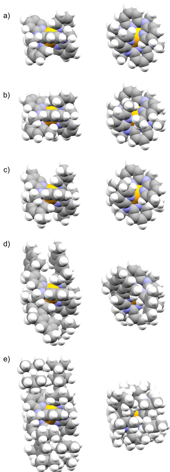
Fig. 1 Space-filling models of (a) [\text{Cr}(\text{ddpd})_2]^{3+} , (b) [\text{Cr}(\text{ddpd}^{5\text{Me}})_2]^{3+} , (c) [\text{Cr}(\text{ddpd}^{5\text{Mes}})_2]^{3+} , (d) [\text{Cr}(\text{ddpd}^{5\text{Mes}})_2]^{3+} and (e) [\text{Cr}(\text{ddpd}^{5\text{Tripp}})_2]^{3+} from DFT calculations demonstrating the increasing shielding of the chromium center (orange: Cr, blue: N, grey: C, white: H). Left: front view, right: top view.
