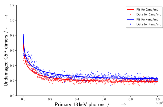
Fig. 8 Change in the number of undamaged G5P dimers with dependence on the amount of primary X-ray photons with 13 keV incident energy. The curve is a fit according to eqn (6).
