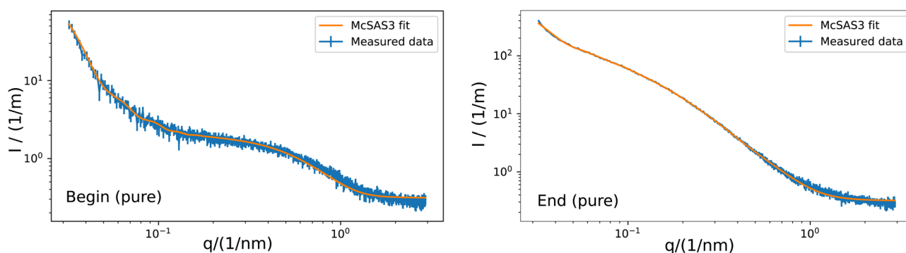
Fig. 3 Example of the fitting of a sphere model with McSAS3 to the obtained scattering curve of the G5P sample without scavenger at a concentration of 4 \text{ mg mL}^{-1} . McSAS at the beginning (left) and end (right) of the measurement. Hereby q is the scattering vector and I the intensity. Additional curves and fits are shown in the ESI.† The related histograms are shown in Fig. 4.
