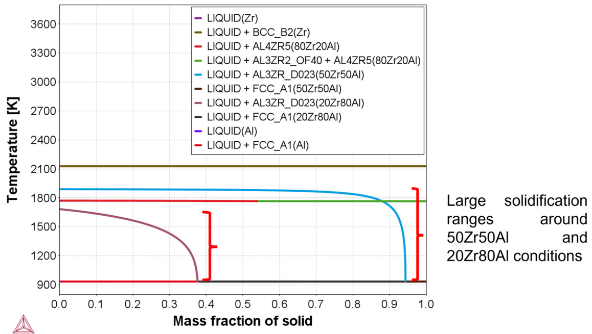
Fig. 18. Scheil solidification [44] for five conditions with different Al-Zr phases namely Zr (100 wt% Zr), 80Zr20Al (80 wt% Zr, 20 wt% Al), 50Zr50Al (50 wt% Zr, 50 wt% Al), 20Zr80Al (20 wt% Zr, 80 wt% Al), Al (100 wt% Al). Solidification range can be up to 1000 K (for 50Zr50Al condition), which could cause heavy solidification cracking.
