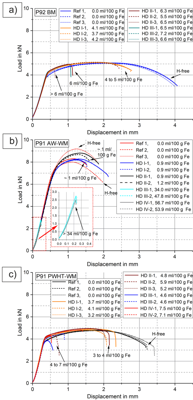
Fig. 4 Load displacements curves for the different HD levels vs. hydrogen free reference: a) P92 BM, b) P91 AW-WM, and c) P91 PWHT-WM
