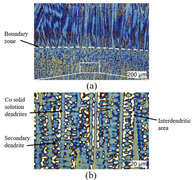
Fig. 2 Light microscopic images of microstructure of \text{CoCr}_{26}\text{Ni}_9\text{Mo}_5\text{W} (a) and detail of dendritic microstructure (b) [24]
