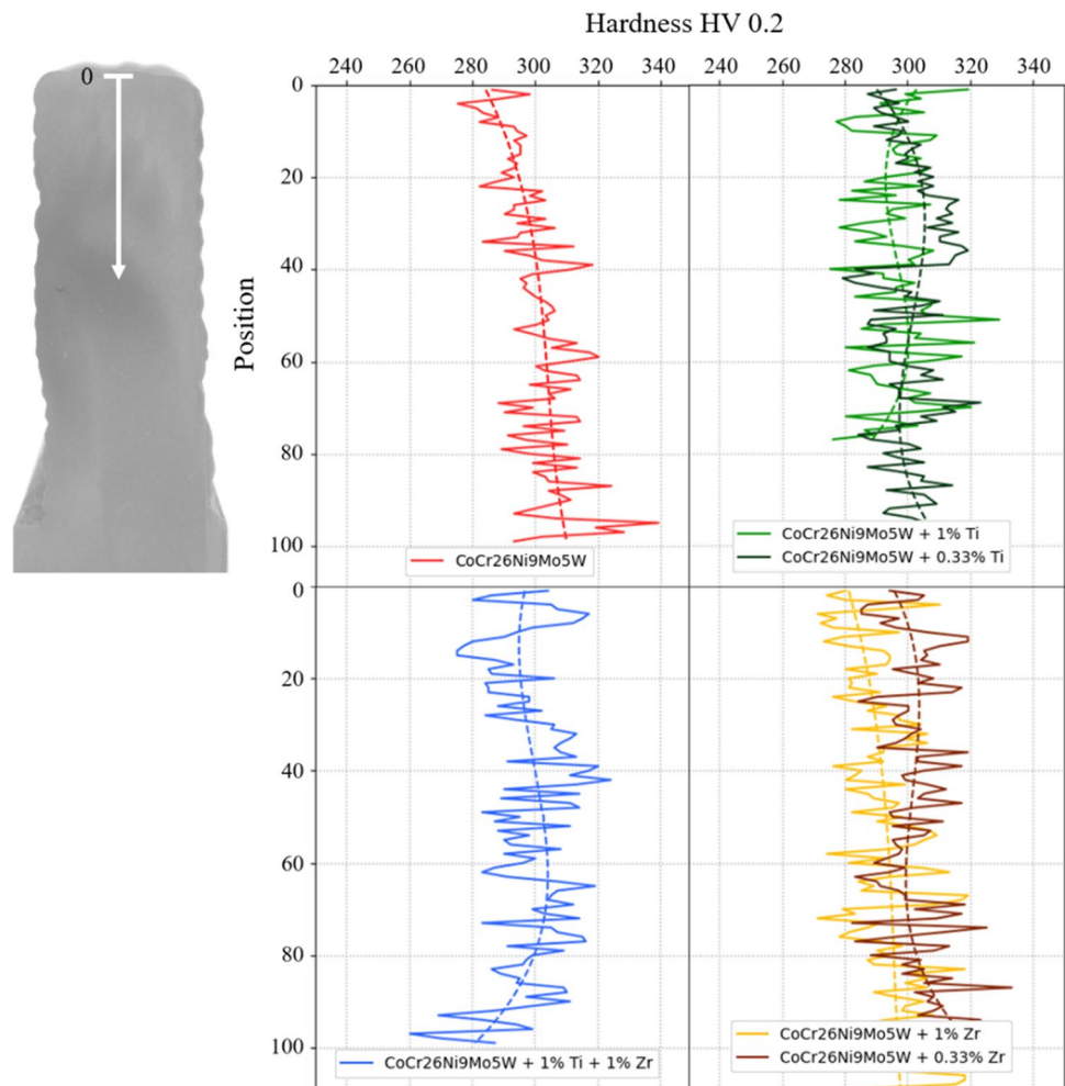
Fig. 6 Hardness measurement series HV 0.2 over the entire cross section
