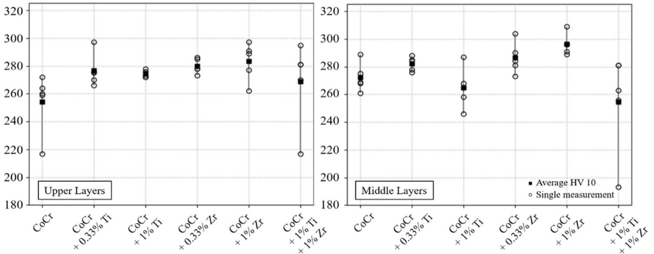
Arithmetic mean of hardness HV 10
