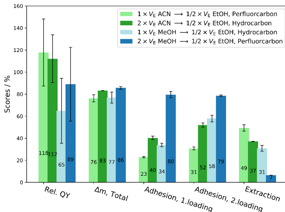
Figure 4. Relative quantum yields (QY) to QDs feed solution and separated mass differences ( \Delta m ) at different parameter conditions using 70–90 \mu\text{m} \text{SiO}_2 -beads. Error bars result from standard deviations running the parameter conditions twice and with respect to the quantum yield from linear regression errors.
