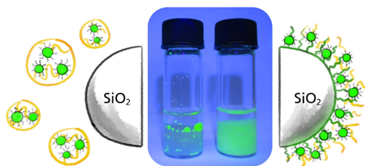
Figure 2. Raw synthesis solution in contact with MeOH and untreated non-porous SiO 2 -beads ( left ) or hydrocarbon surface-modified SiO 2 -beads ( right ).
