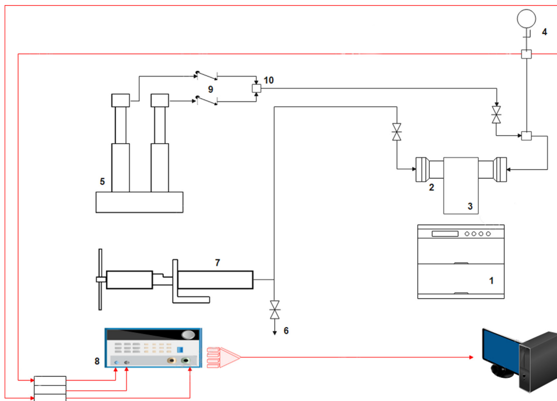
Fig. 1. View of the experimental vibrating-wire rig: (1) thermostatic bath, (2) pressure vessel with the vibrating-wire sensor, (3) magnet, (4) pressure transducer, (5) ISCO syringe pumps, (6) Mity Mite valve (pressure controller), (7) pressure generator (a manually operated spindle press), (8) lock-in amplifier, (9) check valves and (10) mixing point. The modification of the apparatus is mainly in the pressure line with the addition of the back-pressure system.
