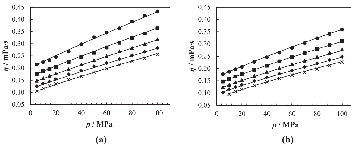
Fig. 4. Experimental viscosities of the system (CO 2 (1) + n -pentane (2)) at: a) x_1 = 0.1 and b) x_1 = 0.3 as function of pressure at different temperatures: (●) 293.15 K; (■) 313.15 K; (▲) 333.15 K; (◆) 353.15 K; (×) 373.15 K. The lines represent the calculated values using the modified VFT model with the parameters given in Table 8.
