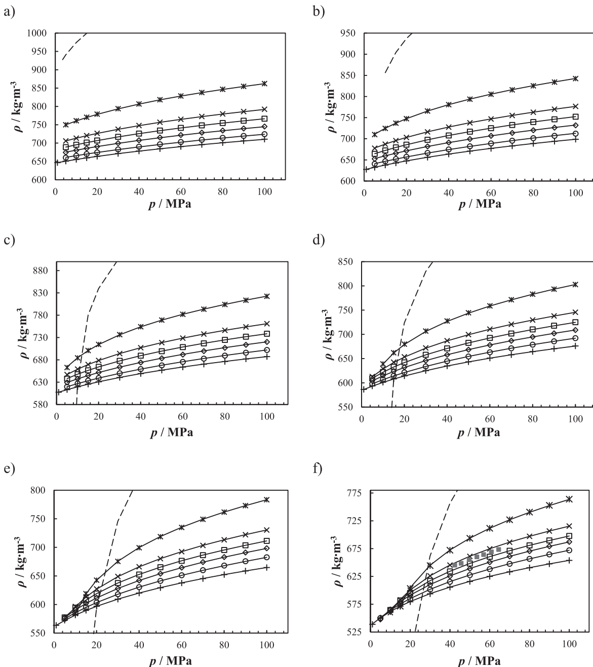
Fig. 2. Experimental density of the system (CO 2 (1) + n -pentane (2)) as function of pressure, at temperatures: (a) 273.15 K; (b) 293.15 K; (c) 313.15 K; (d) 333.15 K; (e) 353.15 K; (f) 373.15 K and different compositions: (+) x_{\text{CO}_2} = 0 ; (○) x_1 = 0.1 ; (◊) x_1 = 0.2 ; (◻) x_1 = 0.3 ; (×) x_1 = 0.4 ; (*) x_1 = 0.6 . Lines represent the calculated values using a modified Tammann-Tait equation with the corresponding parameters given in Table 4. The dashed lines (---) represent pure CO 2 [24]. In f), experimental data of Kiran et al. [7] at x_1 \sim 0.3 are represented using filled grey symbols.
