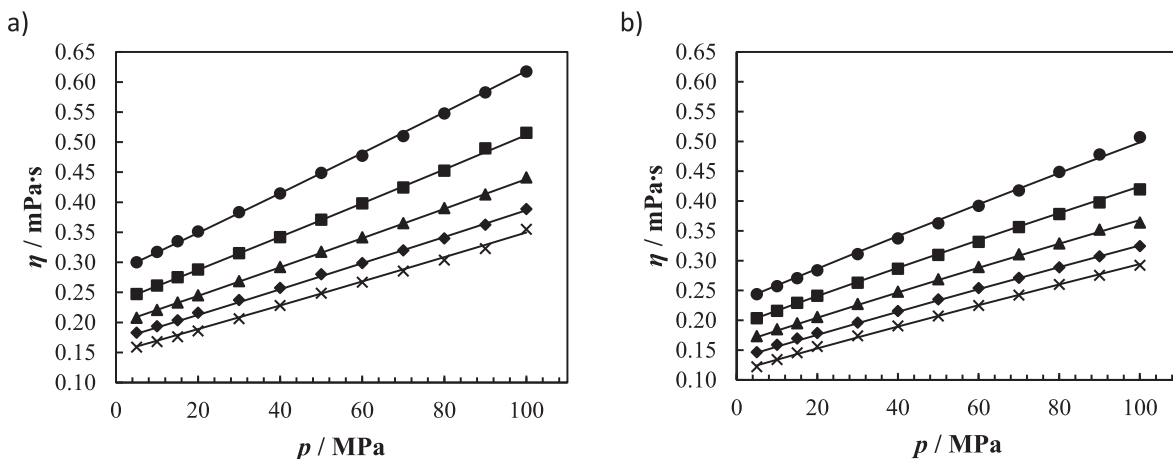
Fig. 5. Experimental viscosities of the system (CO 2 (1) + n -hexane (2)) at: a) x 1 = 0.1 and b) x 1 = 0.3 as function of pressure at different temperatures: (●) 293.15 K; (■) 313.15 K; (▲) 333.15 K; (◆) 353.15 K; (×) 373.15 K. The lines represent the calculated values using the modified VFT model with the parameters given in Table 8.
