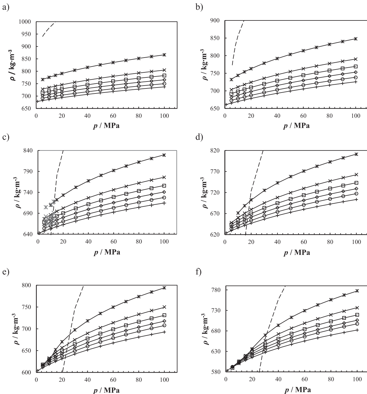
Fig. 3. Experimental density of the system ( \text{CO}_2 (1) + n -hexane (2)) as function of pressure, temperatures: (a) 273.15 K; (b) 293.15 K; (c) 313.15 K; (d) 333.15 K; (e) 353.15 K; (f) 373.15 K and at different compositions: (+) x_1 = 0 ; (○) x_1 = 0.1 ; (◊) x_1 = 0.2 ; (◻) x_1 = 0.3 ; (×) x_1 = 0.4 ; (※) x_1 = 0.6 . Lines represent the calculated values using a modified Tammann-Tait equation with the corresponding parameters given in Table 4. The dashed lines (---) represent pure \text{CO}_2 [24]. In c), experimental data of Tolley et al. [10] are represented using grey symbols.
