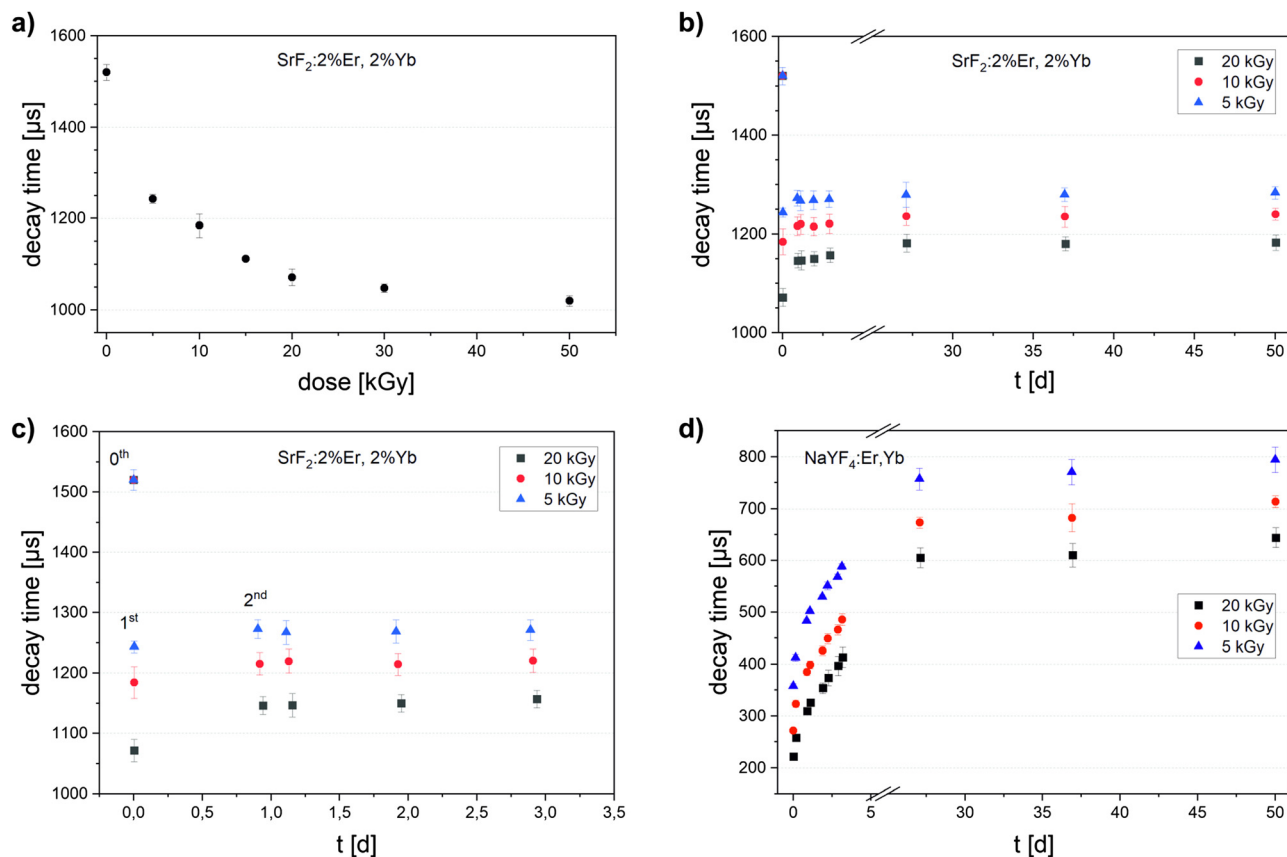
Fig. 4 (a) Luminescence decay times of SrF 2 : 2 mol% Er 3+ , 2 mol% Yb 3+ after 200 keV electron irradiation with the given doses (dose response curve). (b) Luminescence decay times of SrF 2 : 2 mol% Er 3+ , 2 mol% Yb 3+ irradiated with 5, 10 and 20 kGy up to 50 days after irradiation (fading curve). (c) The same fading curve as before, shown only for the first three days (0 th measurement represents decay times before irradiation). (d) Fading curve of NaF 4 :Er,Yb up to 50 days after irradiation for comparison; decay time before irradiation is 1224 μs ± 8 μs (not shown in the diagram).
