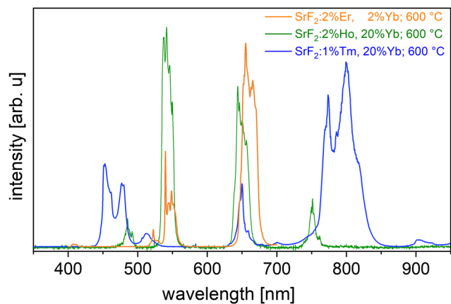
Fig. 5 UC emission of Yb doped SrF 2 codoped with Er (orange line), Holmium (green line) and Thulium (blue line).
