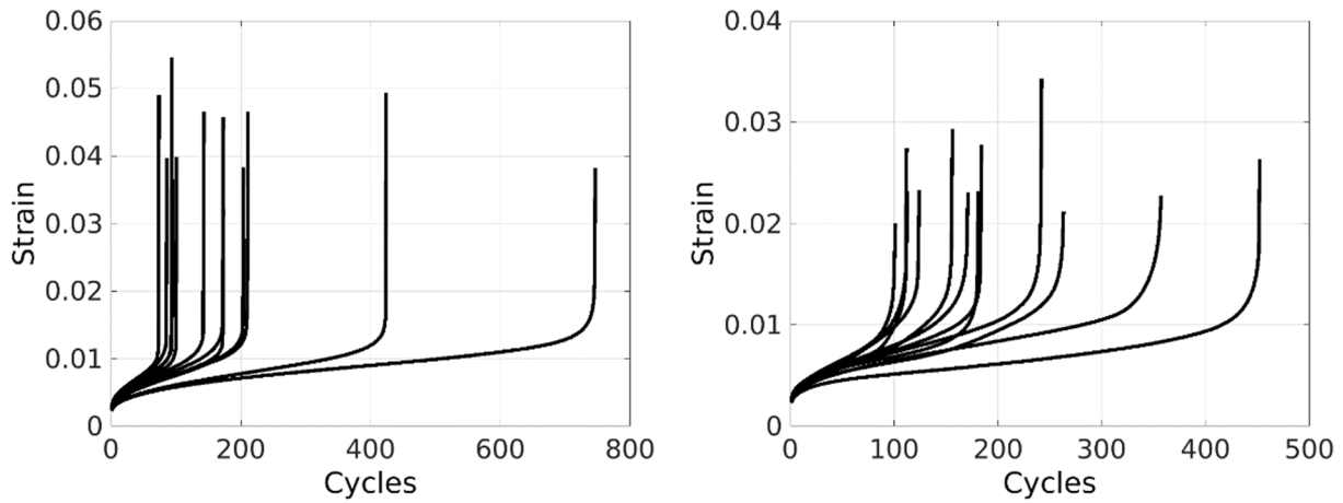
Fig. 5. Typical \epsilon - N curves for steel-fiber reinforced concretes with different fiber content (plain concrete on the left; H15 on the right). From [44].
