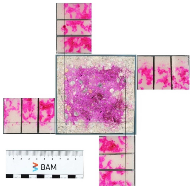
Figure 7. Results of the gel-pad shaped indicator compared to the results of the sprayed application of phenolphthalein solution on a concrete specimen.
