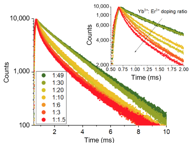
Figure 3 Summarized normalized \text{Yb}^{3+} decay curves and corresponding doping ratio normalized to the \text{Er}^{3+} concentration. The reduced \text{Yb}^{3+} decay time indicates higher energy transfer rates for \text{Er}^{3+} concentrations approaching the \text{Yb}^{3+} doping concentrations. The \text{Yb}^{3+} luminescence was excited at 978 nm and recorded at 1000 nm.
