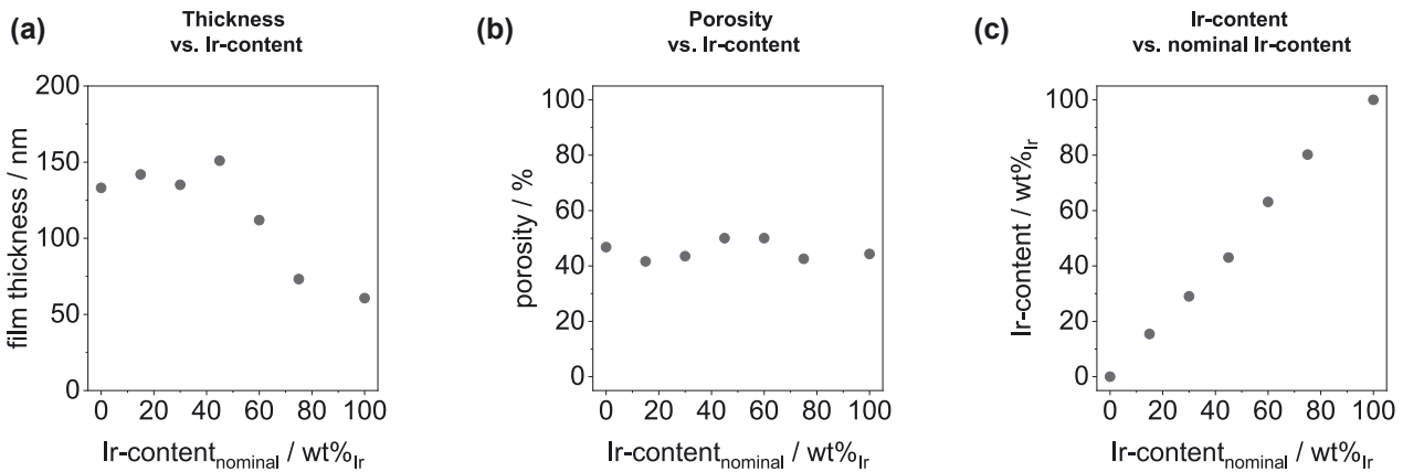
Figure 7: Results of ellipsometric modeling of mesoporous \text{IrO}_x - \text{TiO}_y films with Ir-contents between 0 wt% Ir ( \text{TiO}_y ) and 100 wt% Ir ( \text{IrO}_x ). a) Film thickness versus the nominal Ir-content. b) Porosity and c) Ir-content as a function of the nominal Ir-content.
