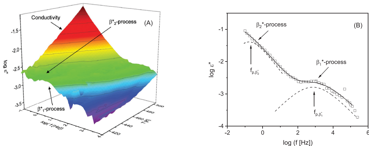
FIGURE 3 (A) Dielectric loss versus frequency and temperature for exo-PNBSi. (B) Fit of two HN-functions to the dielectric loss data of exo-PNBSi at T = 486 K. The solid line is the whole fit function where the dashed lines represent the contributions of the individual processes
