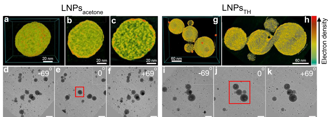
Figure 5. 3D-reconstructed images of LNPs. (a) 3D-reconstructed structure, (b, c) cross-sectional views, and (d–f) the corresponding 2D TEM projections at -69^\circ , 0^\circ , and +69^\circ extracted from the tilt series of \text{LNPs}_{\text{acetone}} . (g) 3D-reconstructed structure, (h) cross-sectional view, and (i–k) the corresponding 2D TEM projections at -69^\circ , 0^\circ , and +69^\circ extracted from the tilt series of \text{LNPs}_{\text{THF}} . The scale bars in TEM projections are 100 nm. The red boxes mark the particles used for 3D reconstruction. The 10 nm fiducial gold particles were used as markers (see the red dots in (g)). Note that the electron density bar is used to indicate the density difference in one analysis, and thus the density differences of the two kinds of LNPs cannot be compared to each other.
