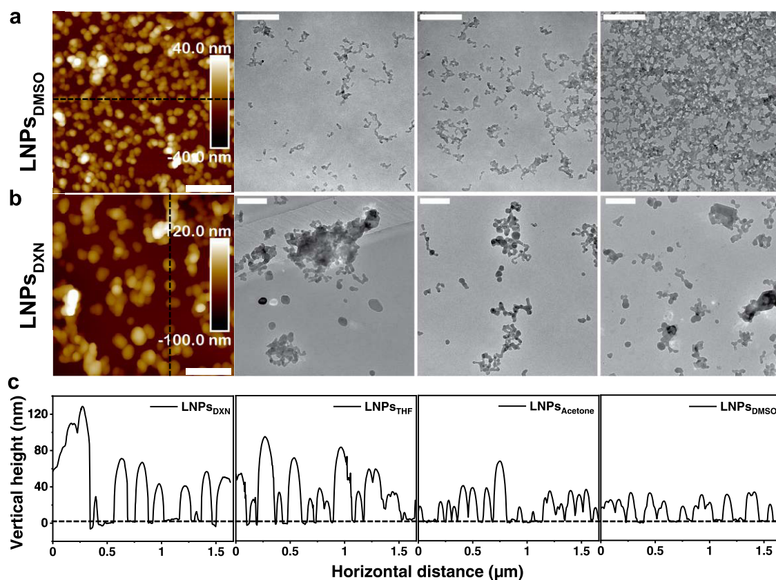
Figure 3. AFM and TEM images of (a) \text{LNPs}_{\text{DMSO}} and (b) \text{LNPs}_{\text{DDXN}} . All scale bars are 400 nm. (c) Cross-sectional height profiles of the LNPs corresponding to the black dashed lines in (a) and (b) and in Figure 1a,d. Areas with as many as possible single particles were chosen for the line scan.
