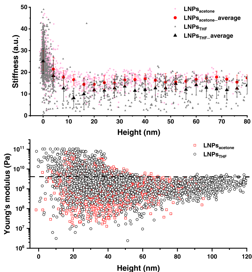
Figure 6. (a) Stiffness as a function of the height of LNPs acetone and LNPs THF , measured with ImAFM. The stiffness data were taken from the very top region of the particles. (b) Young's modulus as a function of the height of LNPs acetone and LNPs THF determined with AFM in Force Volume mode. The height was manually corrected to start from around 0 nm. The dashed line at 4 GPa roughly distinguishes the E resulting from the substrate (above 4 GPa) and the particles (below 4 GPa).
