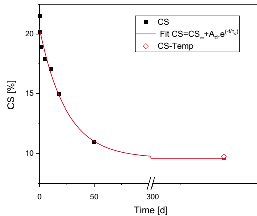
Fig. 4 Evolution of the recovery of EPDM aged at 125 °C for 10 d over time and its corresponding fit
