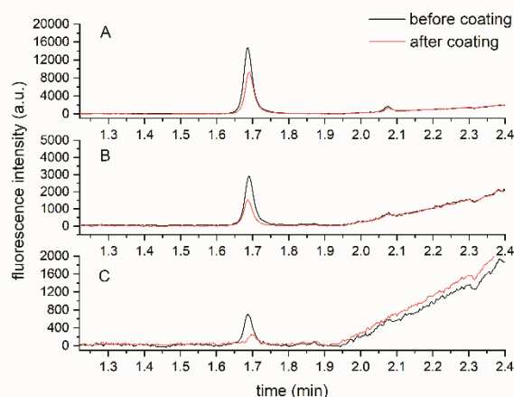
Figure 7: Chromatograms of supernatant hydrolysates, taken before and after coating from large (A), small (B) and no excess (C) samples
