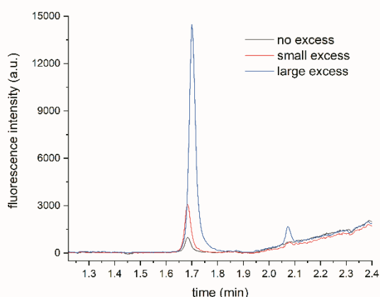
Figure 6: Chromatograms of supernatant hydrolysate samples taken before the coating of all three different IgG concentrations used; Tyr signal at approx. 1.7 min, Phe signal at 2.08 min
