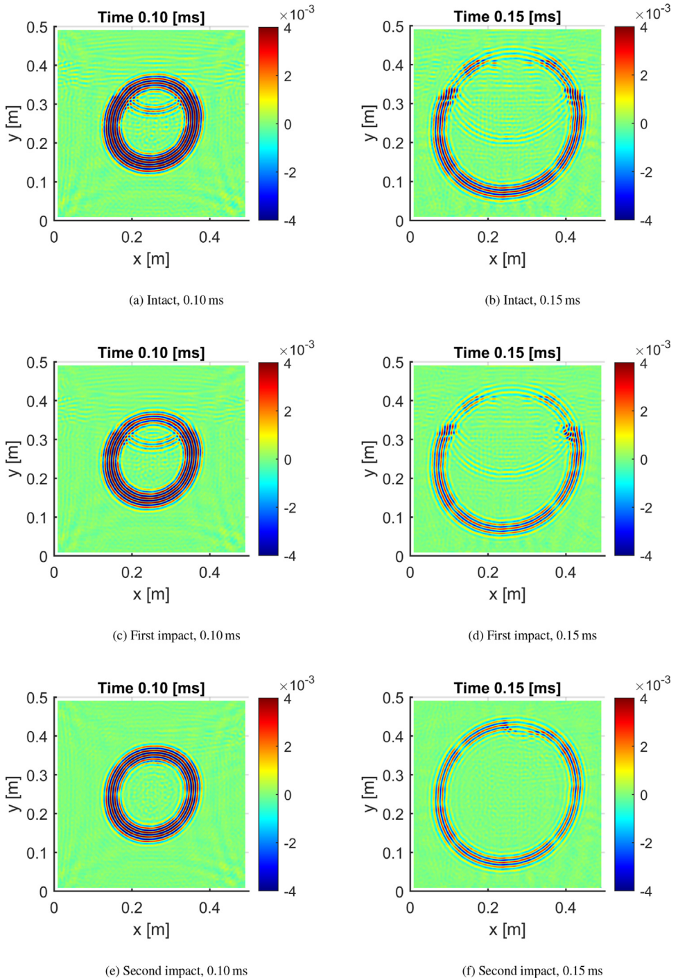
Fig. 9. Exemplary frames of propagating waves for the case of intact plate, first impact and second impact.
