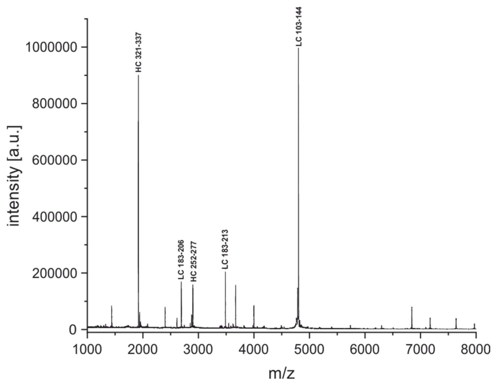
Figure 7. MALDI-TOF fingerprint spectrum of NIST-mAb 8671 after 15 minutes of incubation with TCEP at 99 °C, followed by 15 minutes of incubation with trypsin at 55 °C. The five most intense peptide peaks are assigned to the sequence of the NIST antibody in the spectrum (HC heavy chain, LC light chain). Sequence assignment was possible for most peaks (see SI, Figure S5). The sequence coverage was around 65%.
