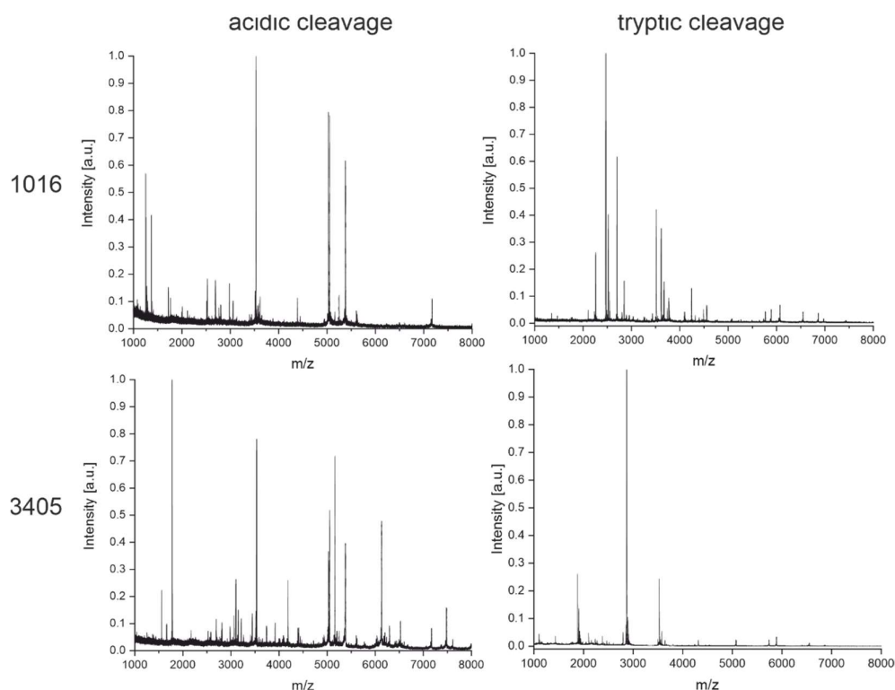
Figure 9. MALDI-TOF fingerprint spectra of the monoclonal antibodies 1016 and 3405 were obtained from cleavage with diluted sulfuric acid for 30 minutes at 99 °C and tryptic digestion for 15 minutes at 55 °C. Antibodies 1016 and 3405 originated from different immunizations but have similar light chain and intact masses. However, some obvious differences showed up in the fingerprints based on acidic cleavage and tryptic digest.
