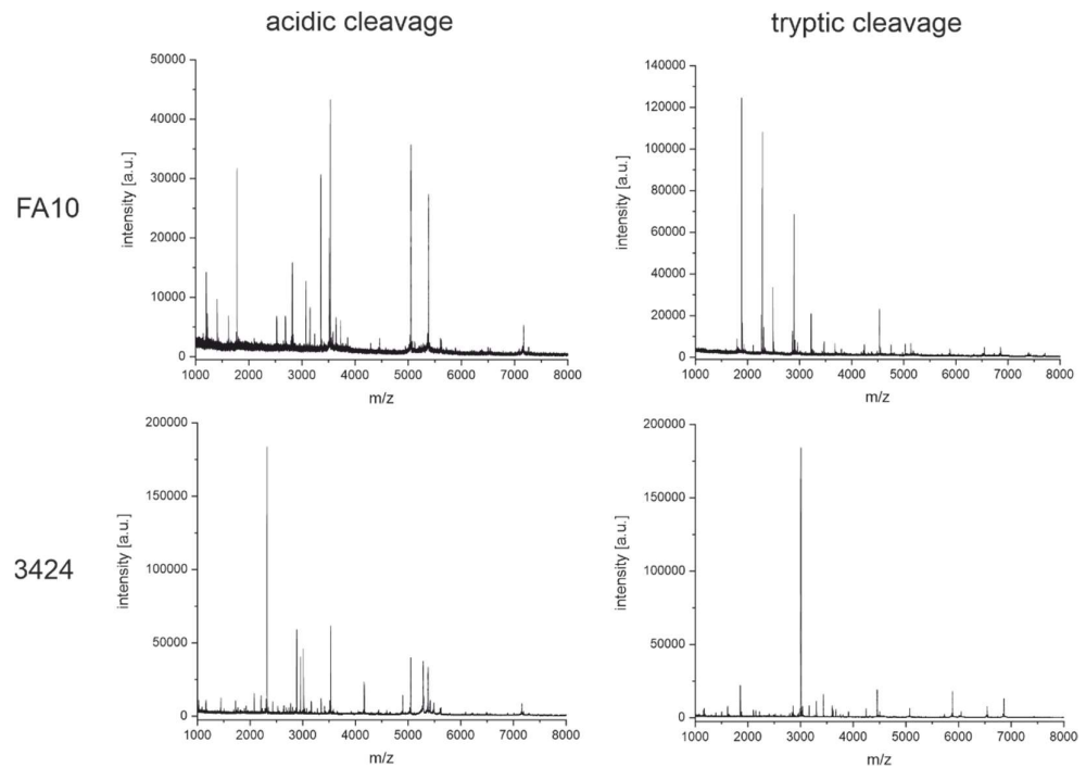
Figure 8. MALDI-TOF fingerprint spectra of the monoclonal antibodies FA10 and 3424 were obtained from cleavage with diluted sulfuric acid for 30 minutes at 99 °C and tryptic digestion for 15 minutes at 55 °C. Antibodies FA10 and 3424 originated from different immunizations and have different light chain and intact masses.
