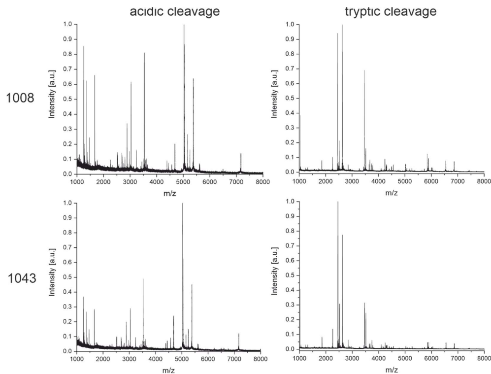
Figure 10. MALDI-TOF fingerprint spectra of the monoclonal antibodies 1008 and 1043 were obtained from cleavage with diluted sulfuric acid for 30 minutes at 99 °C and tryptic digestion for 15 minutes at 55 °C. Antibodies 1008 and 1043 originated from the same immunization and turned out to be identical after a later hybridoma sequencing. The similarity is evident even by a brief visual inspection.
