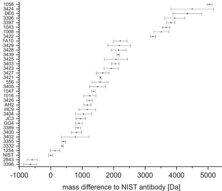
Figure 2. Intact masses of anti-SARS-CoV-2 antibodies relative to NIST-mAb 8671 given with a confidence level of 95%
