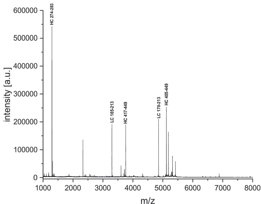
Figure 6. MALDI-TOF fingerprint spectrum of NIST-mAb 8671 after 30 minutes of incubation with diluted sulfuric acid and TCEP at 99 °C. The five most intense peptide peaks are assigned to the sequence of the NIST antibody in the spectrum (HC heavy chain, LC light chain). Sequence assignment was possible for most peaks, including variable and hypervariable regions (see Figure S4). The sequence coverage was around 61%.
