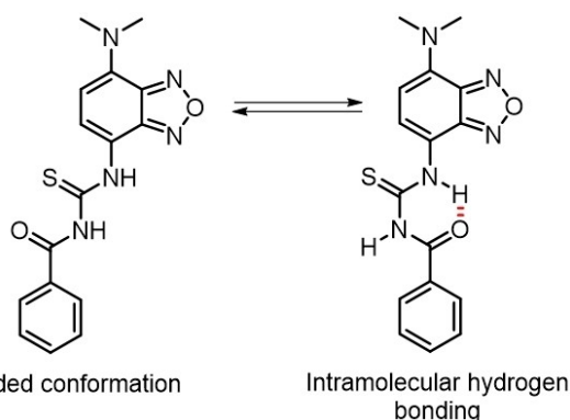
Figure 2. Conformational equilibrium between the extended and the intramolecularly hydrogen-bonded conformations of 2a .
