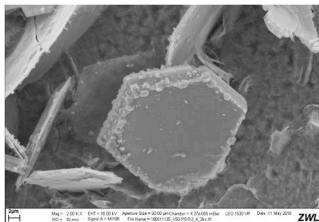
Fig. 12. SEM-image of pseudo-hexagonal hydrocalumite (AFm) inside the pores of the treated mortar prisms.
