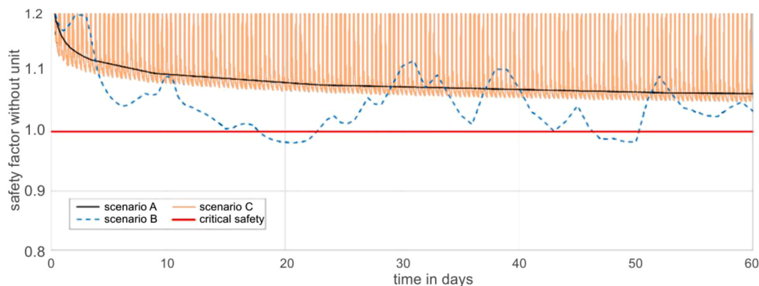
Fig. 8. Temporal development of the dimensionless safety factor (SF) within the first 60 days of injection. SF below 1.0 (red line) indicates a possible occurrence of tensile failure within the cap rock. Different injection scenarios are considered: constant (A), varying (B) and cyclically fluctuating (C) injection rate.
