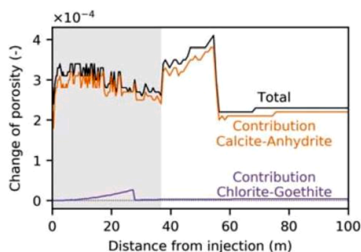
Fig. 15. Simulated changes of total porosity including individual contributions of the coupled mineral reactions after one year of injection exemplarily shown for a scenario using an “averaged” sandstone composition of Buntsandstein from the North German Basin and a CO 2 stream containing SO 2 , NO 2 , O 2 and H 2 in temporally varying concentrations.
