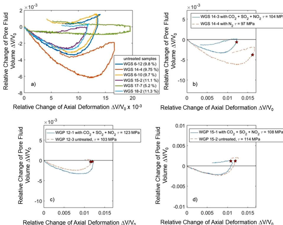
Fig. 16. Pore fluid volume changes of different sandstone cores as a function of the axial deformation in triaxial tests (different colours indicate individual samples; figures modified after Menezes, 2019) and dependence of the pore fluid volume change on the core drilling direction and the sample treatment – a) untreated samples (cores drilled perpendicular to bedding; measured effective porosities are given in the legend); b) samples treated in brine with \text{N}_2 (orange line) or with \text{CO}_2 containing \text{NO}_2 and \text{SO}_2 (70 ppm v each; blue line) (core drilled perpendicular to the bedding). c) and d) untreated samples (orange line) and samples loaded with \text{CO}_2 containing \text{NO}_2 and \text{SO}_2 (70 ppm v each; blue line) (cores drilled parallel to bedding). Red star symbols indicate the point of the maximum shear stress of the sample before mechanical failure.
