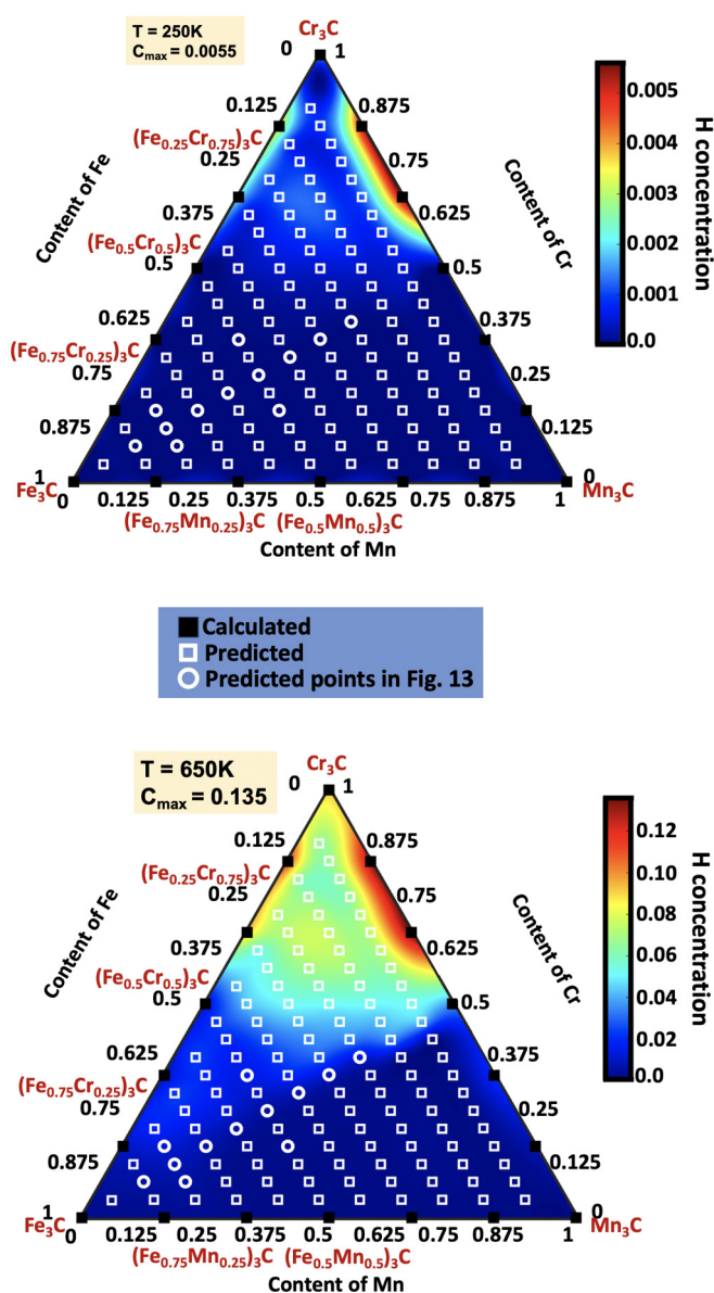
FIG. 14. Heat maps of H concentration in (\text{Fe,Cr,Mn})_3\text{C} carbides at two different temperatures is plotted in the form of a Gibbs triangle. The black-filled squares along the border of the triangle correspond to the H concentration values obtained using ab initio calculations in binary-metal carbides and the white nonfilled squares inside the triangle represent the H concentration values in ternary-metal carbides from the machine learning model. The white nonfilled circles in the triangle correspond to the test set of the model. The projected heat maps of the H concentration are obtained by employing a cubic interpolation scheme on the data points.
