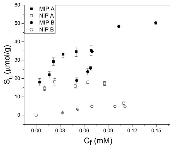
Fig. 4 Batch rebinding measurements using UV-vis absorption spectroscopy for two polymer compositions using solutions of nafcillin sodium salt in PBS ( \text{pH} = 7.4 ).
