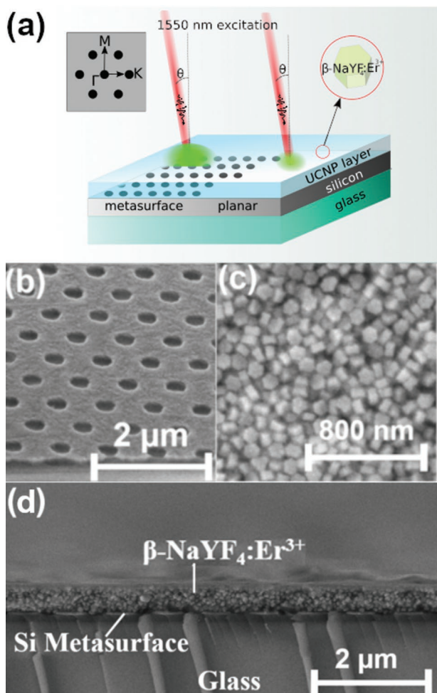
Figure 2. Photon UC system designed to convert near-infrared (1550 nm) to visible light. a) Schematic of the UC system comprised of a silicon metasurface covered with a \beta\text{-NaYF}_4\text{:Er}^{3+} NP layer as well as geometrical details of the experimental setup designed for UC enhancement investigation. b) Scanning electron microscopy (SEM) image of the covered silicon metasurface, taken at viewing angle 30^\circ . c) Top view on the \beta\text{-NaYF}_4\text{:Er}^{3+} NP layer on metasurface. d) SEM cross-section image of a 660 nm thick \beta\text{-NaYF}_4\text{:Er}^{3+} NP layer covering the silicon metasurface, respectively. The planar appearance on top of the NP layer can be regarded as an artefact due to charging effects during the SEM measurements.
