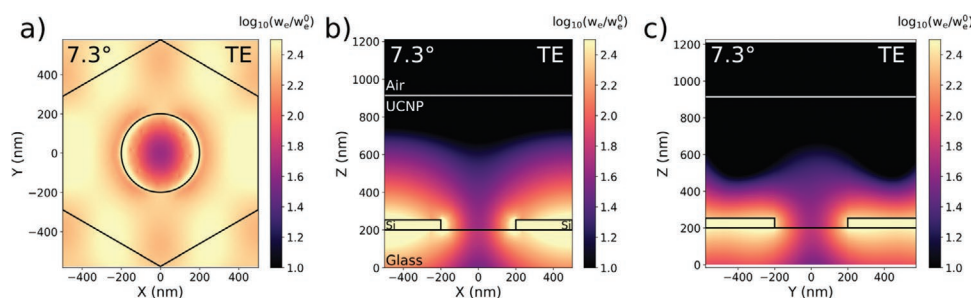
Figure 4. The logarithm of the electric field energy density in cross-sectional planes of the simulated hexagonal unit cell of the metasurface for TE-polarized light incident with an angle of 7.3° at 1551 nm. a) The x - y -plane is evaluated at z = 1 nm above the silicon surface. The b) x - z - and c) y - z -planes are evaluated at y = 0 and x = 0 , respectively. In part (b), the materials of the sample – UC NP, silicon (Si), and glass – are indicated. w_e and w_e^0 designate the electric field energies in a given region and in the same volume for the incident wave in vacuum, respectively.
