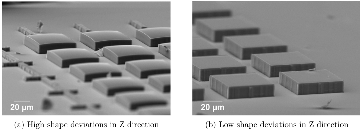
Figure 8. SEM images of structures with (a) high deviations with 90% overlap in hatching and slicing in the upper left and (b) low deviations with 10% overlap in hatching and slicing for the structure in lower left, pre-bake time of 1 h and fabrication direction ‘into the glass’.
