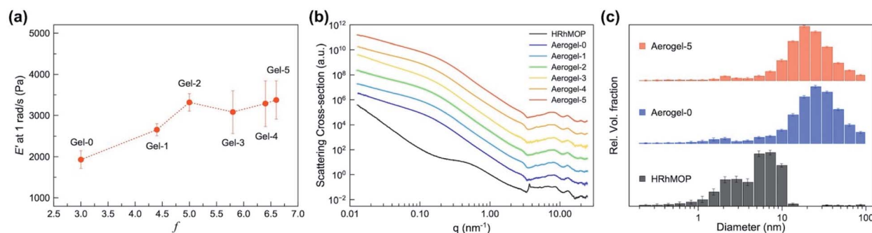
Fig. 3 (a) Evolution of storage Young's modulus ( E' at 1 rad s^{-1} ) of Gel- n as a function of f during repeated aging process. (b) SAXS/WAXS curves of HRhMOP and Aerogel- n (the data was stacked for clarity, all data on an absolute intensity scale can be found in ESI†). (c) Form-free size distributions of HRhMOP, Aerogel-0 and Aerogel-5 extracted from SAXS fits from Monte Carlo method.
