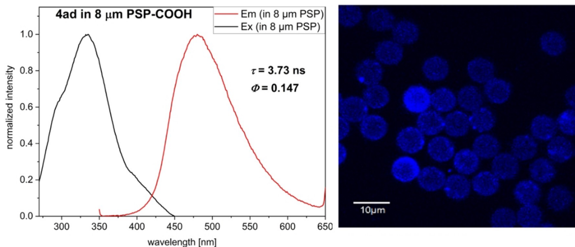
Figure 7. Normalized fluorescence excitation and emission spectra ( \lambda_{\text{exc}} = 401\text{ nm} ) of dispersed 8\text{ }\mu\text{m} -sized PSP loaded with dye 4ad (left) and CLSM image of the dye-loaded PSP (right).
