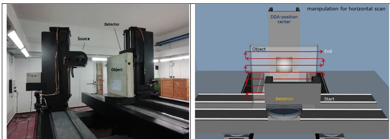
Fig. 5 Left: HEXYTech-equipment for X-ray laminography of large and thick-walled test object. Right: sketch of the horizontal scanning procedure. For each frame position the source and detector move syn-
