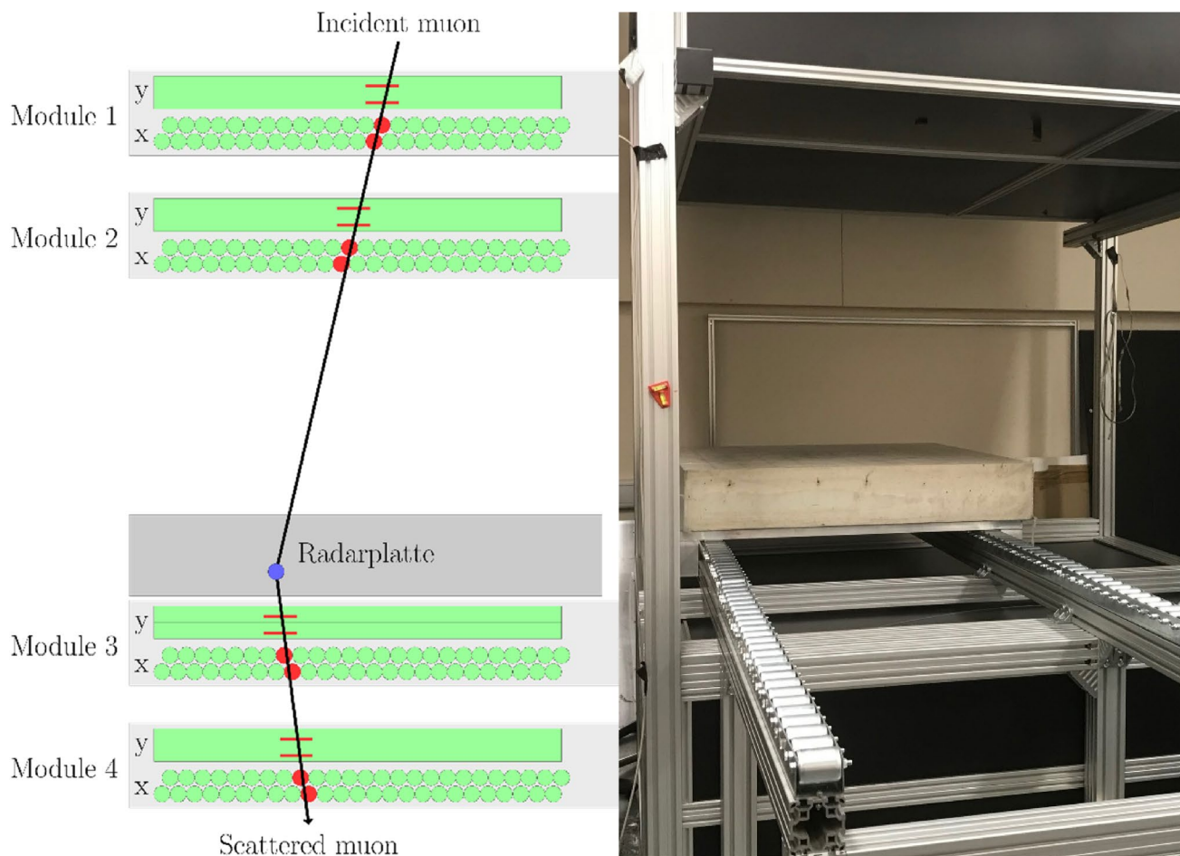
Fig. 2 Muon Imaging. Left: principle of muon tomography. Two detectors above and two detectors below the object were used to trace muon flight paths and scattering, Right: the “Radarplatte” test object inside the Lynkeos Muon Imaging System (MIS)
