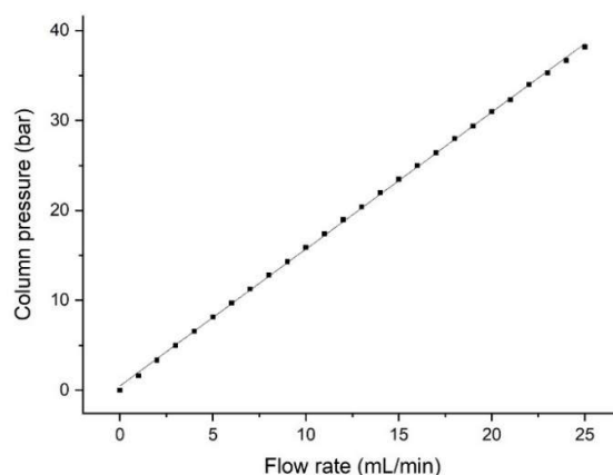
Fig. 5: The system pressure of a VitraPOR 5 column with an increasing flow rate. Due to the flow restrictions of the pump, the upper pressure resistance could not be determined yet. The maximum pressure of 38 bar (550 psi) was tested successfully.
