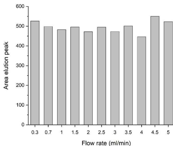
Fig. 8 Examination of the dynamic capacity for IgG of a VitraPOR 5 column. The area of the elution peak was determined in relation to the flow rate. The area was corrected for the different flows.
