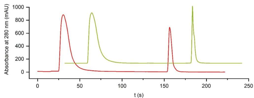
Fig. 7 Effect of a reversed elution on a VitraPOR 5 column. To optimize the peak shape of the eluted product, a reversed elution was tested in comparison to the normal elution in the usual flow direction (red curve). A significant improvement (green curve) of the elution peak can be noticed.
