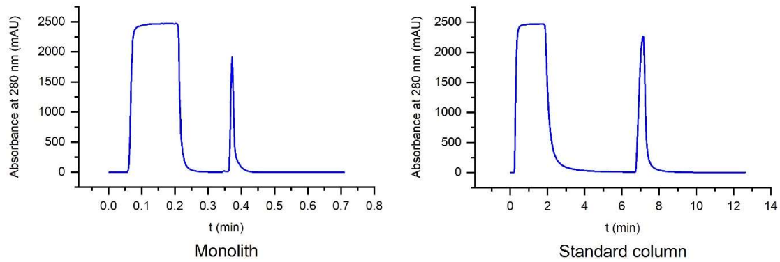
Fig. 10 Comparison of a standard Sephadex-based system with the glass monolith. Due to the very fast separation speed, a productivity gain of 300% (250 mg/hour) can be achieved with the monolith. Please note the very different time scales of the separations. The standard column had a total volume of 1 mL, the monolith around 0.75 mL.
