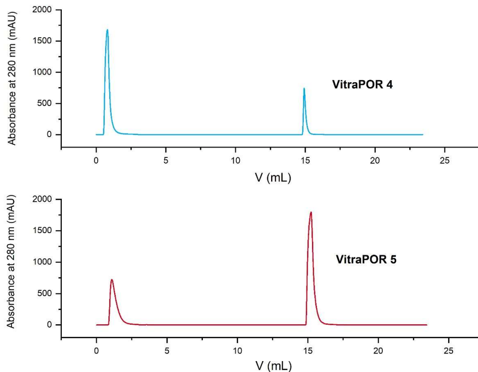
Fig. 11 IgG capacity of the column materials VitraPOR 4 and VitraPOR 5. In both experiments, the same amount of immunoglobulin was injected (5 mg). It can be seen that in the case of the coarser material, a higher void peak and a lower elution peak are obtained in relation to the fine material.
