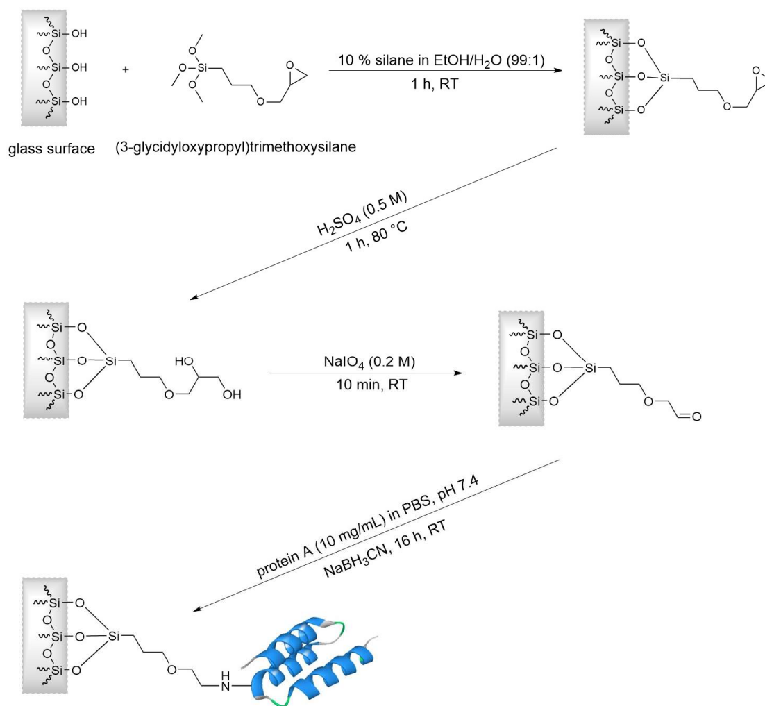
Fig. 4: Scheme of the optimized column conjugation procedure: Surface functionalization with epoxysilane, hydrolysis with sulfuric acid, periodate oxidation, and conjugation of protein A via reductive amination.
