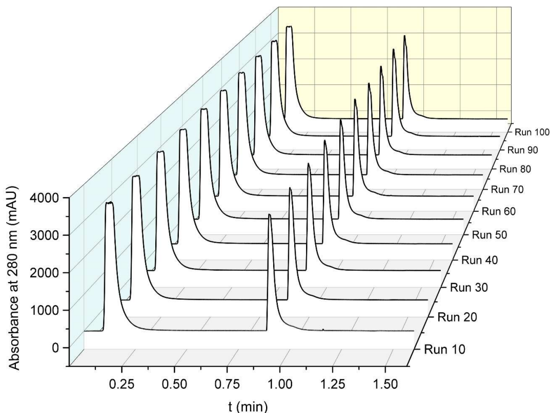
Fig. 9 Representation of 100 extraction/elution cycles of the VitraPOR 5 column. This graph shows an overlay of 100 subsequent runs of an IgG determination from human plasma. Not even a minimal decay of the performance can be noticed. This also means that the cost of the column per run is extremely low.
