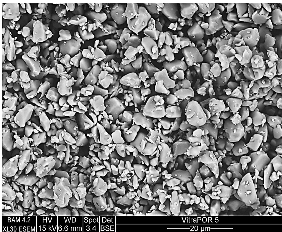
Fig. 1: Environmental scanning electron microscopy (ESEM) of a sintered borosilicate monolith (VitraPOR 5).
