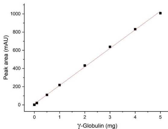
Fig. 14 Calibration line for the quantification of IgG. Different concentrations of bovine IgG were injected directly into the system without a column. There is a linear dependency of the peak area, and the amount of IgG injected.
