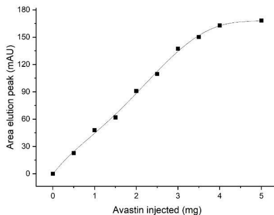
Fig. 6: Saturation curve of the VitraPOR 5 monolith coated with protein A. Increasing elution area in relation to the amount of injected antibody Avastin. It can be seen that about 3 mg of IgG can be bound by the column in a linear way. Based on a linear calibration, a total capacity of about 4 mg IgG per column was determined.
