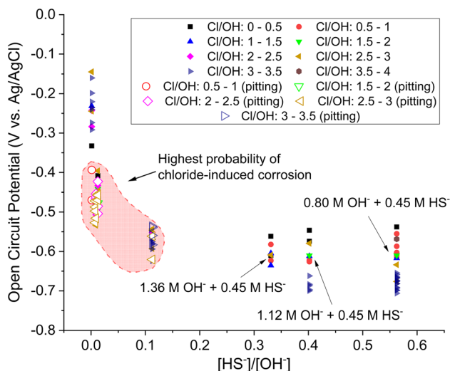
Figure 6 OCP of mild steel exposed to highly alkaline solutions (0.80 M, 1.12 M and 1.36 M OH^- ), with varying concentrations of HS^- (0.001 M, 0.01 M, 0.09 M and 0.45 M) and Cl^- (0–4 in terms of [Cl^-]/[OH^-] ), after 0, 5, 12 and 28 days exposure. The solid symbols denote the steel samples exhibiting no corrosion, whereas the hollow symbols indicate stable or metastable chloride-induced pitting. The transparent red shaded area in (A) indicates the region where the susceptibility to chloride-induced corrosion is the highest.
