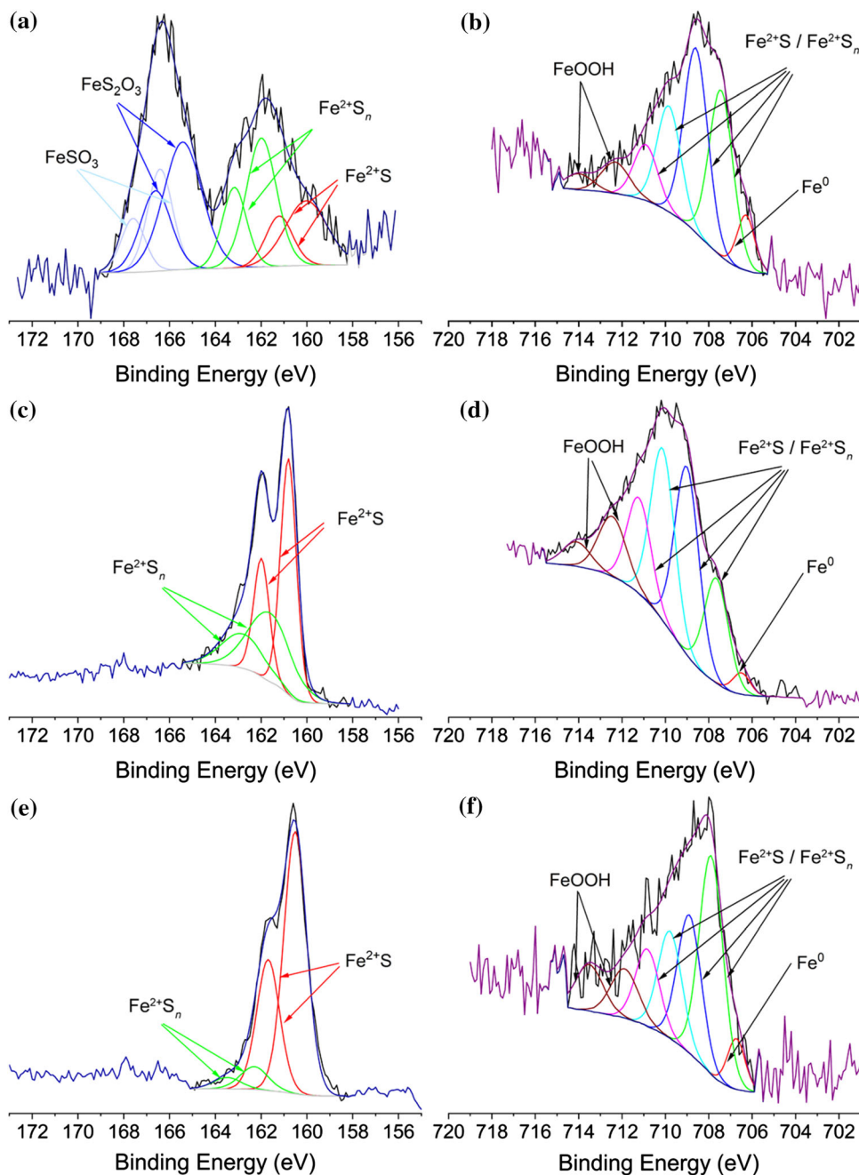
Figure 5 S 2p and Fe 2p_{3/2} XPS spectra of steel specimens exposed to alkaline sulfide solutions for 5 days. a and b show the S 2p and Fe 2p_{3/2} spectra, respectively, for steel immersed in 0.80 M \text{OH}^- + 0.01 M \text{HS}^- ; c and d show the S 2p and Fe 2p_{3/2} spectra, respectively, for steel immersed in 0.80 M \text{OH}^- + 0.09 M \text{HS}^- ; and e and f show the S 2p and Fe 2p_{3/2} spectra, respectively, for steel immersed in 0.80 M \text{OH}^- + 0.45 M \text{HS}^- .
