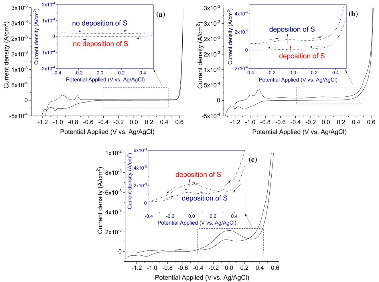
Figure 2 First scan obtained for each sample during the cyclic voltammetry measurements, for mild steel exposed to a 0.80 M OH - , b 0.80 M OH - + 0.01 M HS - and c 0.80 M
