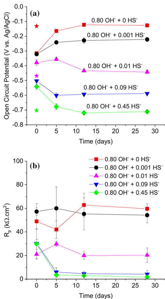
Figure 3 Evolution of the a OCP and b polarization resistance ( R_p ) values determined using the LPR test, for steel immersed in 0.80 M NaOH with varying concentrations of \text{HS}^- as marked, and error bars indicating the results of replicate measurements. The pH values corresponding to these data points are reported in Table S1, Supplementary Information. The data points indicated in (A) by the star symbol refer to the OCP of an inert iridium electrode (experimental details in Supplementary Information Sect. 5) exposed to 0.80 M \text{OH}^- (red star), 0.80 M \text{OH}^- + 0.01 M \text{HS}^- (magenta star), and 0.80 M \text{OH}^- + 0.45 M \text{HS}^- (green star).
