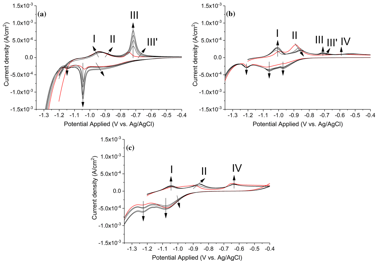
Figure 1 Cyclic voltammograms obtained for mild steel exposed to a 0.80 M \text{OH}^- , b 0.80 M \text{OH}^- + 0.01 \text{ M HS}^- , and c 0.80 M \text{OH}^- + 0.45 \text{ M HS}^- . Data were collected at a sweep rate of 2.5 mV/s. Arrows indicate the current responses in the five scans; each identified response is assigned a Roman numeral for discussion in the text. Data from -1.50 to -1.20 \text{ V} in the 230 anodic sweeps are omitted to enable visibility of all peaks. The red line indicates the first scan, and subsequent scans are represented by black lines.
