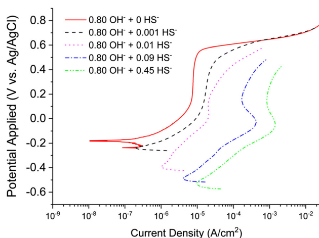
Figure 4 Influence of sulfide (concentrations as marked) on the anodic polarization behavior of obtained mild steel immersed in 0.80 M NaOH.
