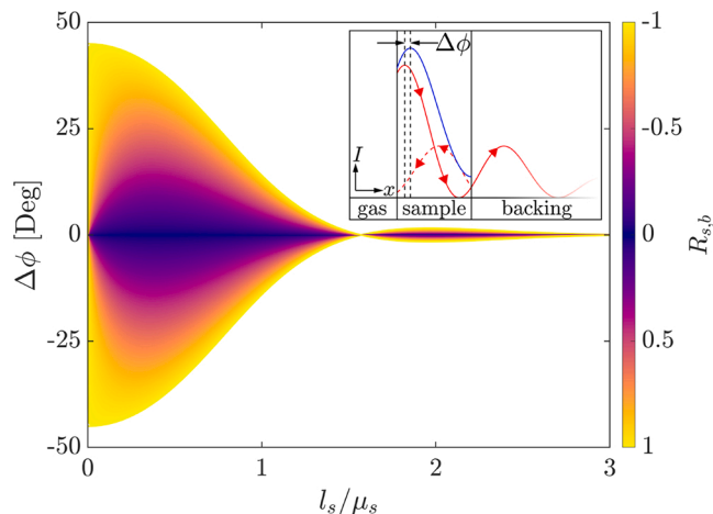
Fig. 1. Theoretical phase shift of the surface temperature for a two-layer system with different thermal reflection coefficients R_{s,b} as a function of the frequency-dependent thermal thickness l_s/\mu_s [15]. The inset is intended to depict the principle of thermal wave interference. (For interpretation of the references to color in this figure legend, the reader is referred to the web version of this article.)
