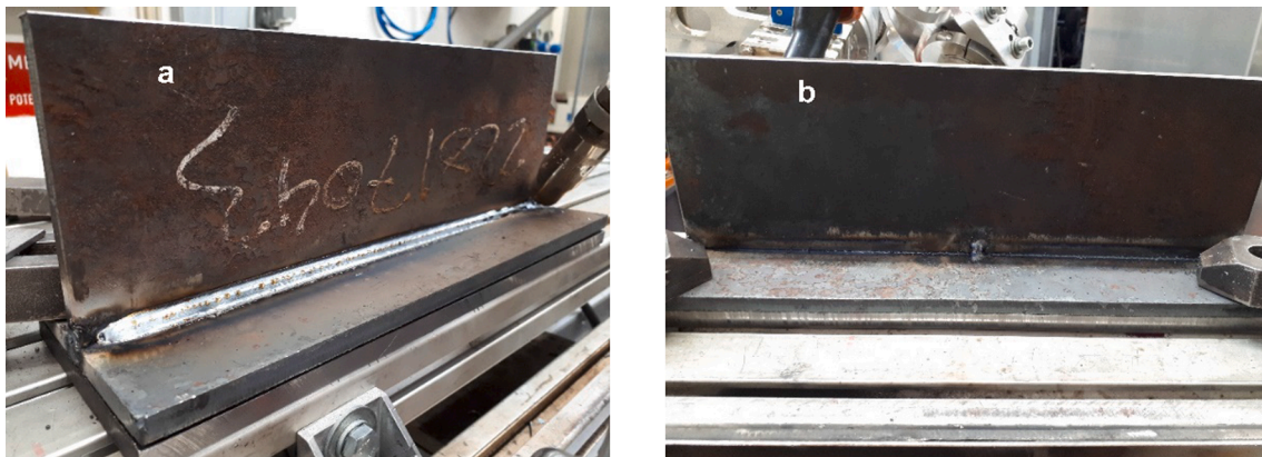
Fig. 7. Image of weld seam of a HLAW T weld. a) Face side; b) Root side.
