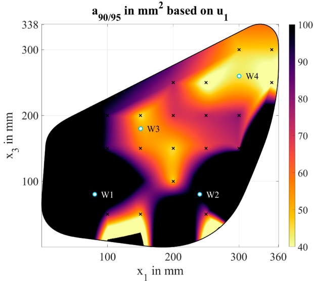
Fig. 13. POD maps obtained by interpolation based on evaluation of u_1 . The transducer W3 was the actuator, and the transducer W4 was the sensor. Top: a_{90} . Bottom: a_{90/95} .
