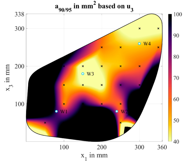
Fig. 14. POD maps obtained by interpolation based on evaluation of u_3 . The transducer W3 was the actuator, and the transducer W4 was the sensor. Top: a_{90} . Bottom: a_{90/95} .
