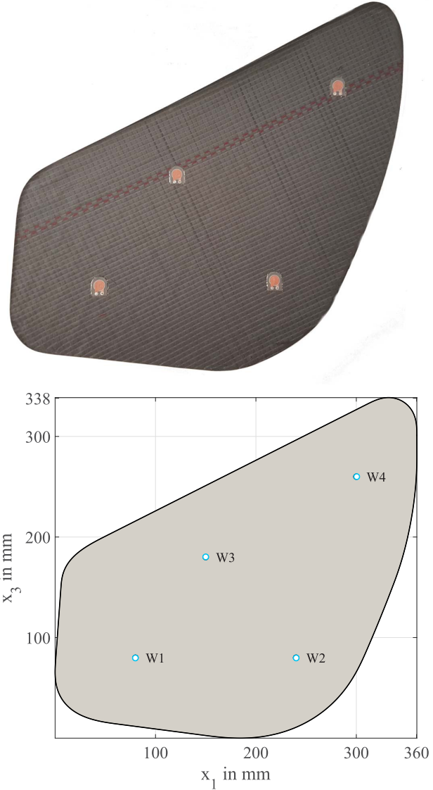
Fig. 3. Top: picture of an automotive component made of CFRP. Bottom: schematic drawing of the 2-D model of the test specimen including marked positions of the PZTs (•).
