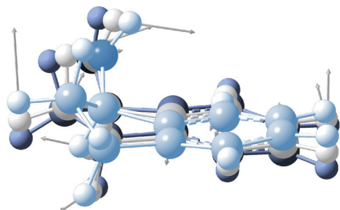
Fig. 5 Normal mode associated with the +116 cm -1 band. The displacement of the vibration is shown with grey arrows. The overlaid molecular structures depict various stages of the vibration.
